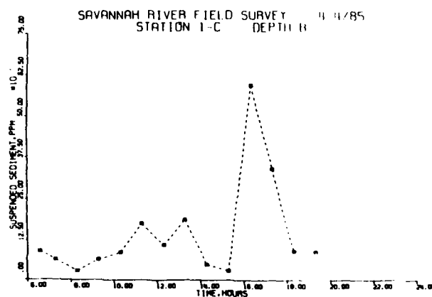
Figure D3. Suspended sediment at Range 1 on right prism line
