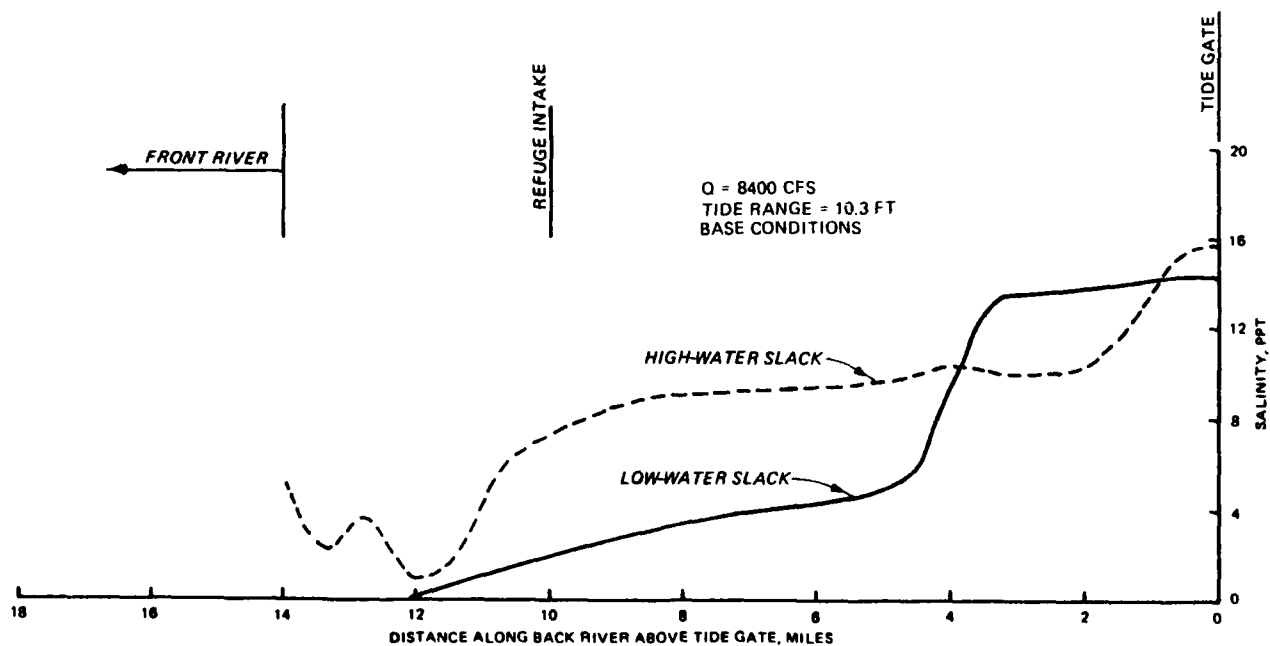
Figure 106. Comparison of high- and low-water slack salinity profiles upstream of the tide gate, 8,400-cfs discharge, 10.3-ft tide range, base conditions
