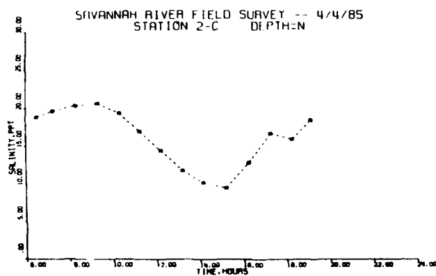
Figure C6. Salinity at Range 2 on right prism line
