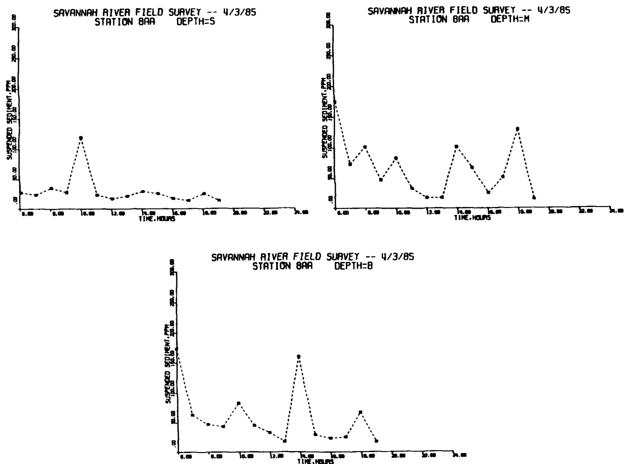
Figure D25. Suspended sediment at Range 8A at center of channel
