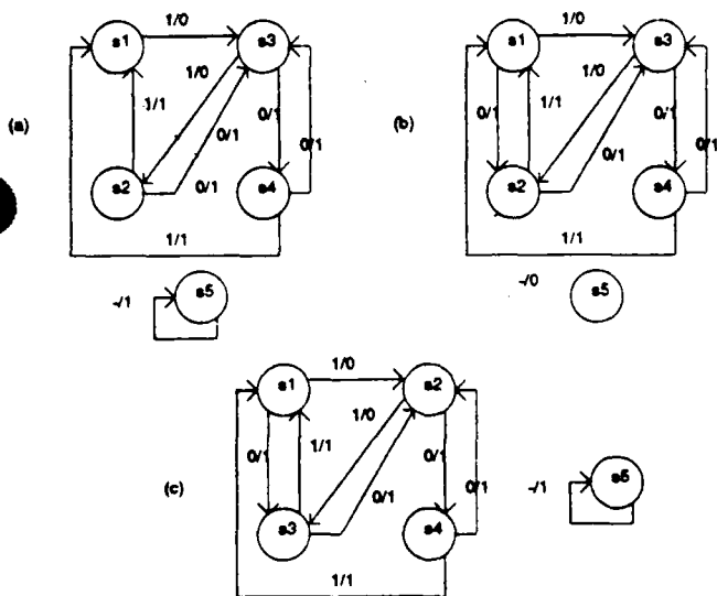
Figure 2: 3 Types of Sequential Redundancies
