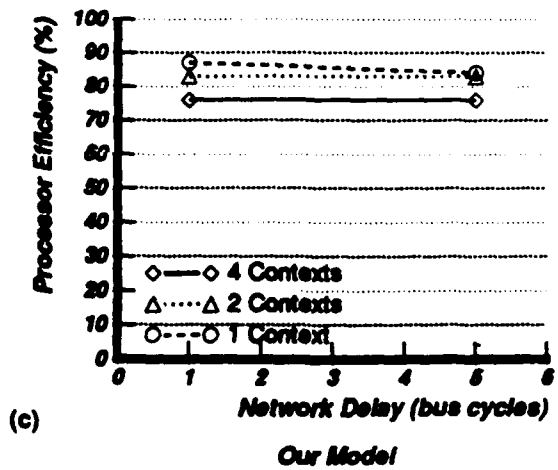
Figure 10: Comparing the model with simulations. (a) Switching overhead 1, (b) 4, and (c) 16.
