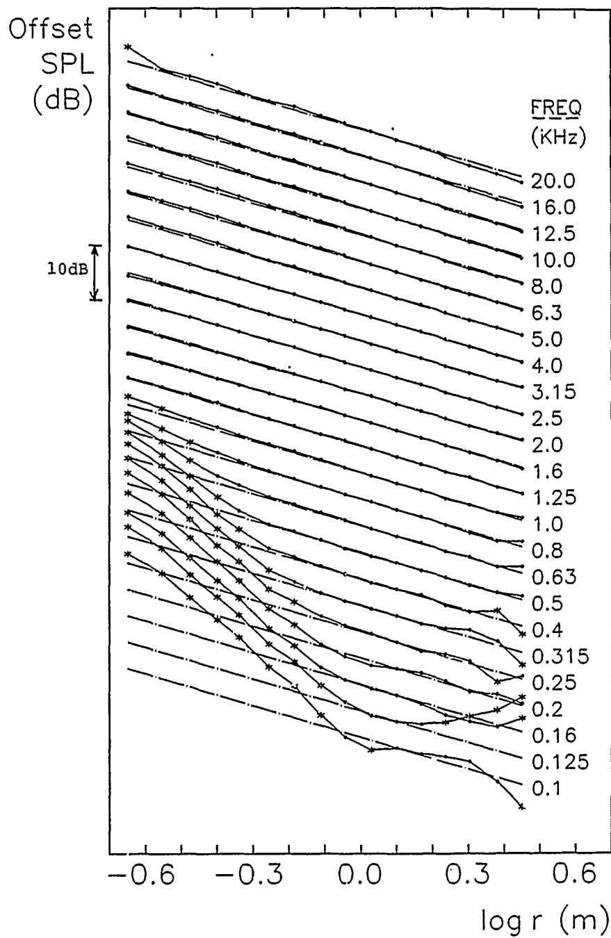
Fig 18 Sound pressure level versus distance from the Reference Sound Source
