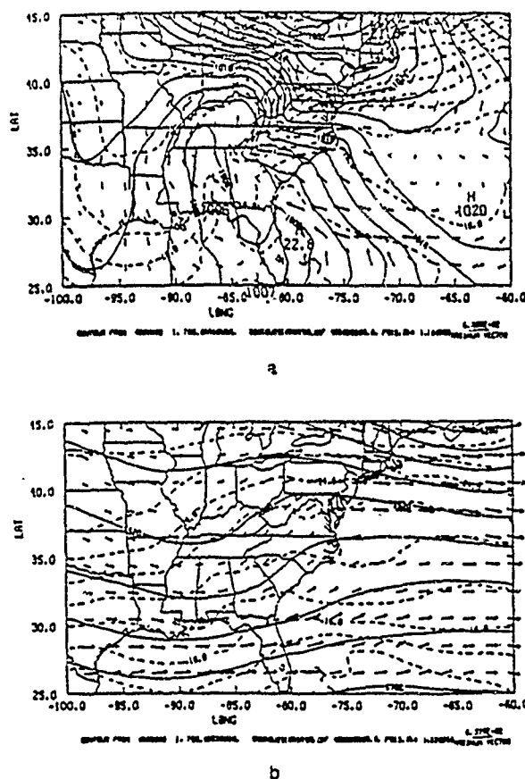
FIG. 4. (a) 24 h surface forecast for exp. 9 (control exp.), valid for 02/11/00Z. (b) Same as Fig. 4a except for 500 mb level.
