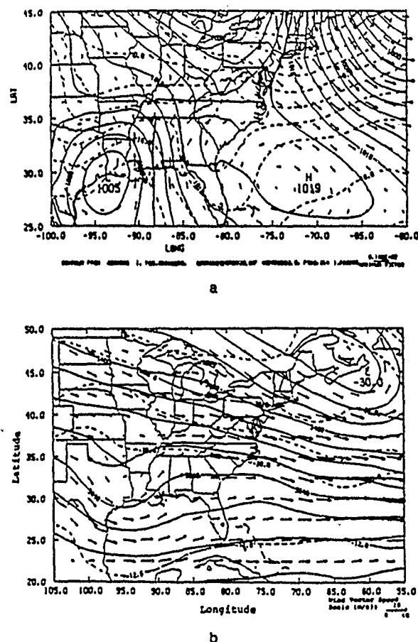
FIG. 1. (a) Rawinsonde enhanced sea level pressure (solid lines, every 2 mb), 1000-mb temperature (dashed line, every 4°C) and 1000-mb wind vector for 1983/02/10/00Z. (b) Rawinsonde enhanced geopotential height (solid lines, every 60 m), temperature (dashed lines, every 4°C) and wind vector (max. 38.4 m s -1 ) at 500 mb level for 1983/02/10/00Z.
