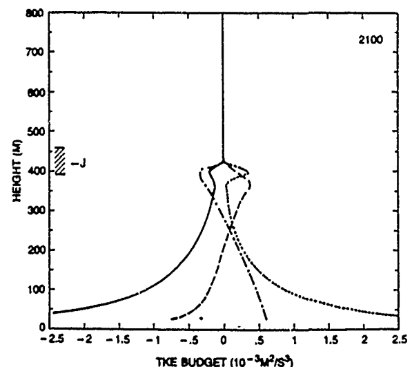
FIG. 14. As in Fig. 11, but for 2100 LST.
