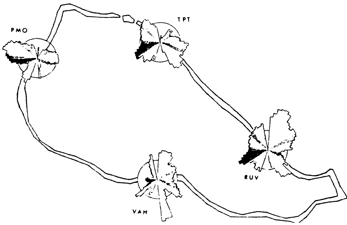
Fig:15 Mb station - Mb means Rangiroa versus azimuth
