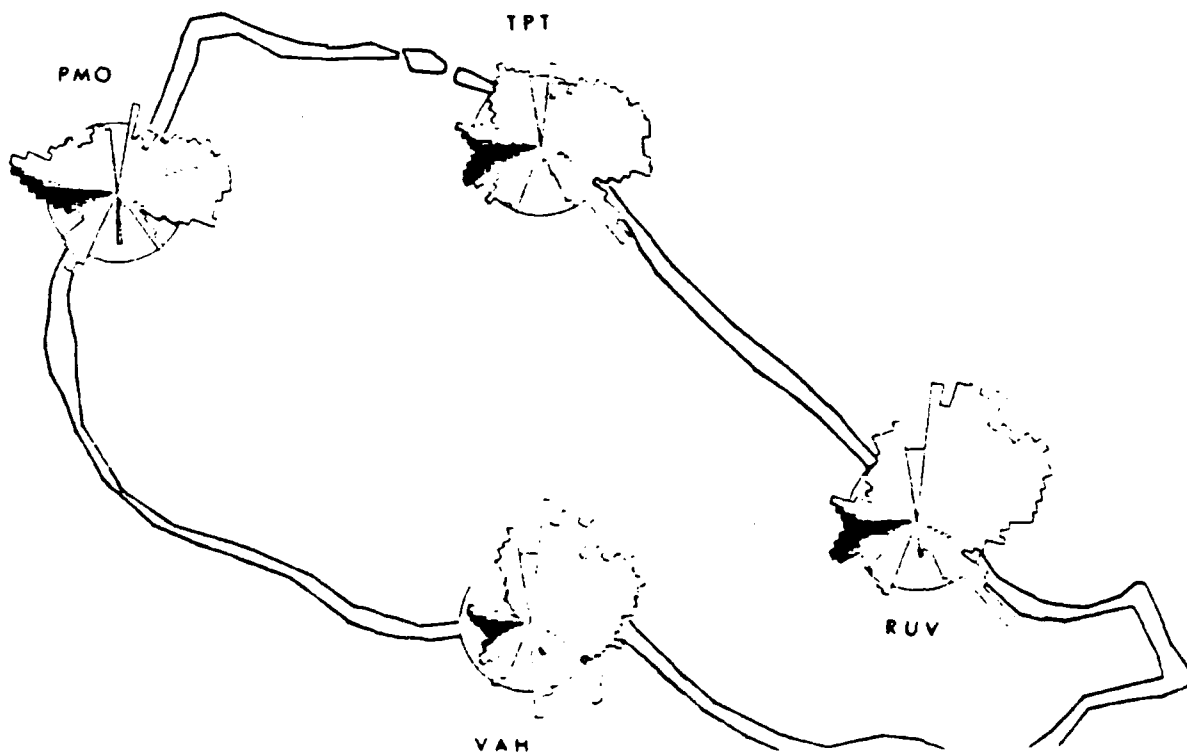
Figure 12 Rangiroa : Mb_{station} - Mb_{USGS} versus azimuth
