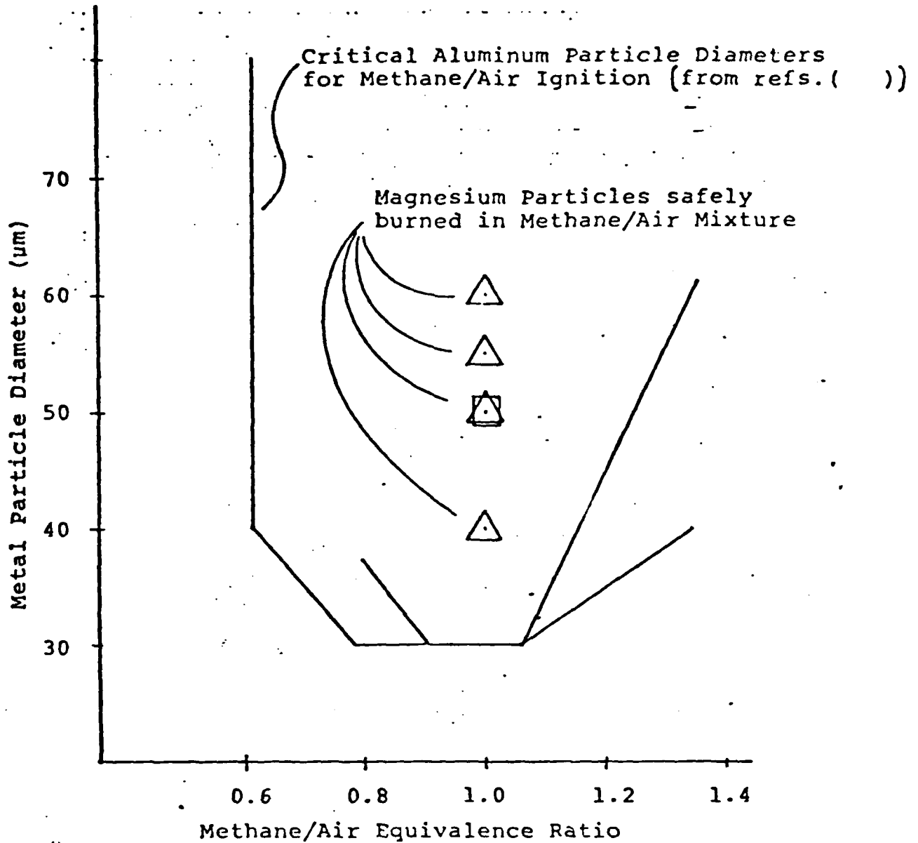
Figure 1: Burning Aluminum and Magnesium Particle Ignition of Methane
