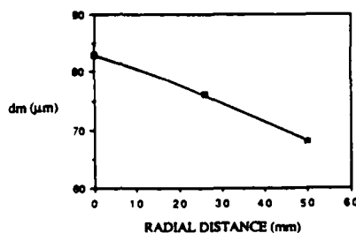
Fig. 13. Variation of mass-median droplet diameter with radial distance from the spray axis; Fe-20% Mn, flight distance = 400 mm.
