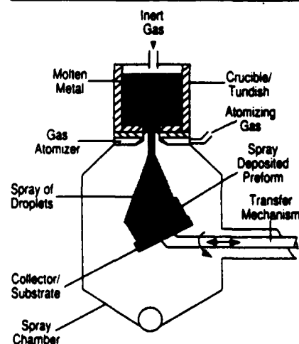
Figure 1. A schematic diagram of the Osprey™ process.
