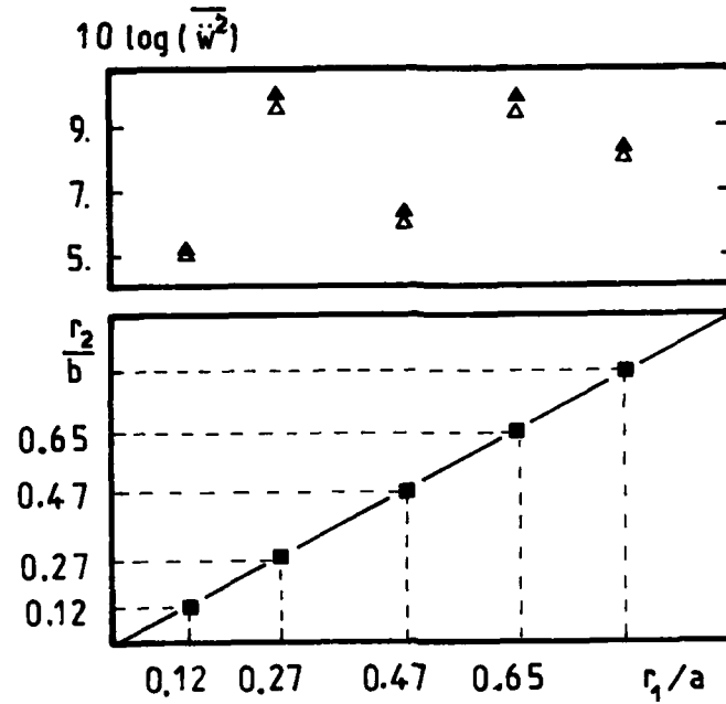
Fig. 3. Comparison between simulated RMS response \blacktriangle and reference response \triangle for different locations on the plate. (Calculation conditions : N = 5 , P = 20 ).
