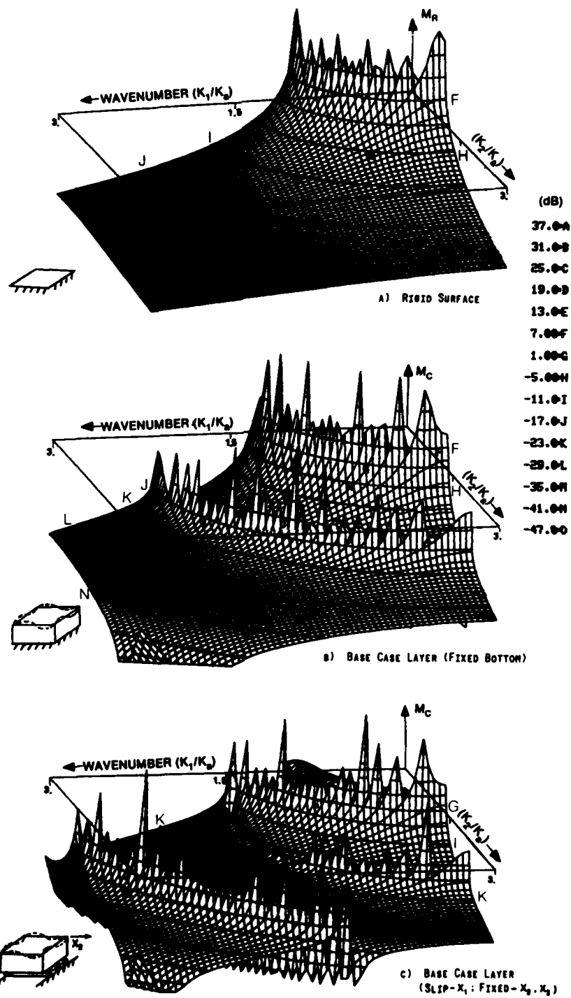
FIGURE 5. CARPET PLOT OF WALL PRESSURE SPECTRUM MULTIPLIER. 20 \log_{10}(|h_p M_p|) . FOR BASE CASE LAYER AT h_0 = \pi/8 .
