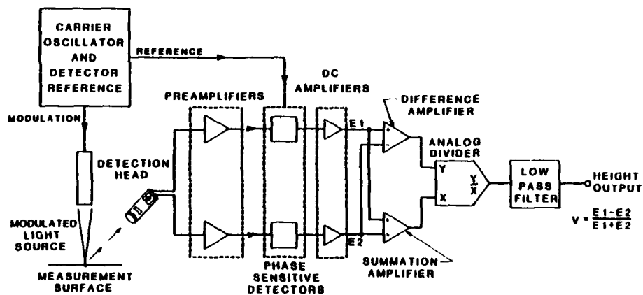
Figure 3. Electro-Optical Displacement Sensor
