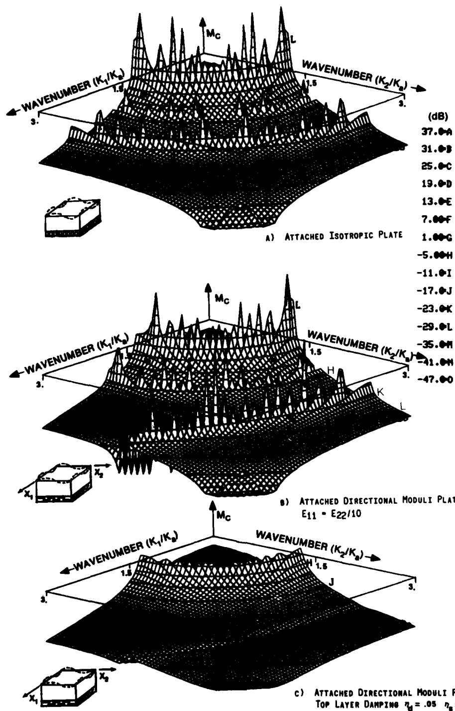
FIGURE 7. CARPET PLOT OF WALL PRESSURE SPECTRUM MULTIPLIER, 20 \log_{10}(|h \cdot M_1|) , FOR BASE CASE LAYER - DIRECTIONAL PROPERTY PLATE ATTACHMENT AT K_0 = \pi/5 .
