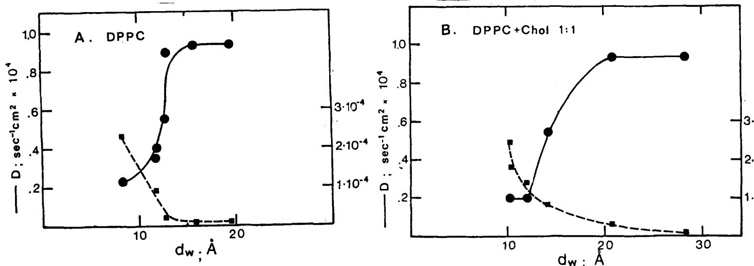
Figure 3. The variation of diffusion coefficient ( \bullet ) and proton-membrane reactivity ( \blacksquare ) as function of the width of the water layer. A) DPPC multilamellar vesicles; B) DPPC+Cholesterol multilamellar vesicles.
