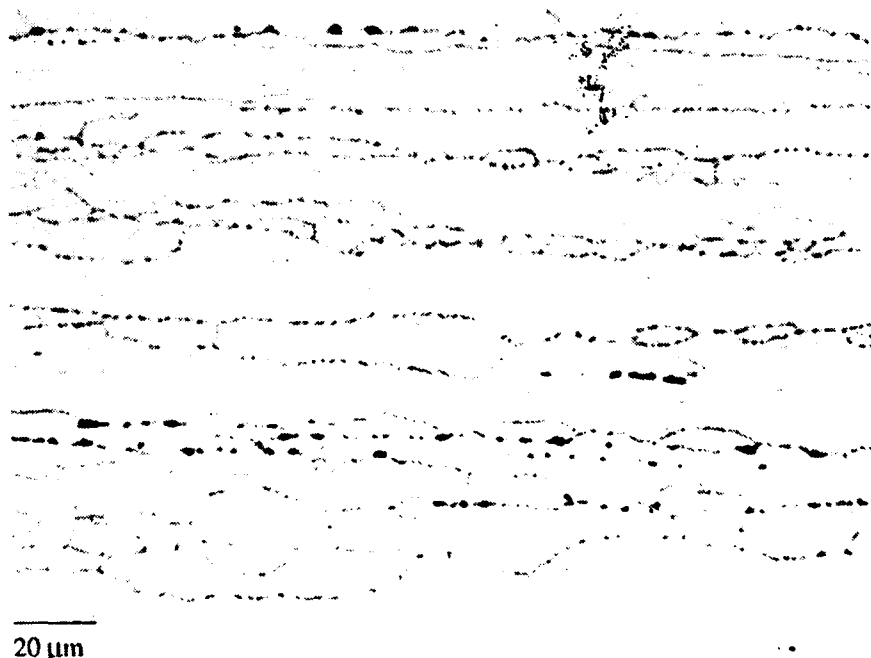
Figure 5. Light micrograph of the longitudinal cross section of the 2090 plate showing coarse \text{T}_2 and \text{Al}_7\text{Cu}_2\text{Fe} precipitates on grain boundaries.
