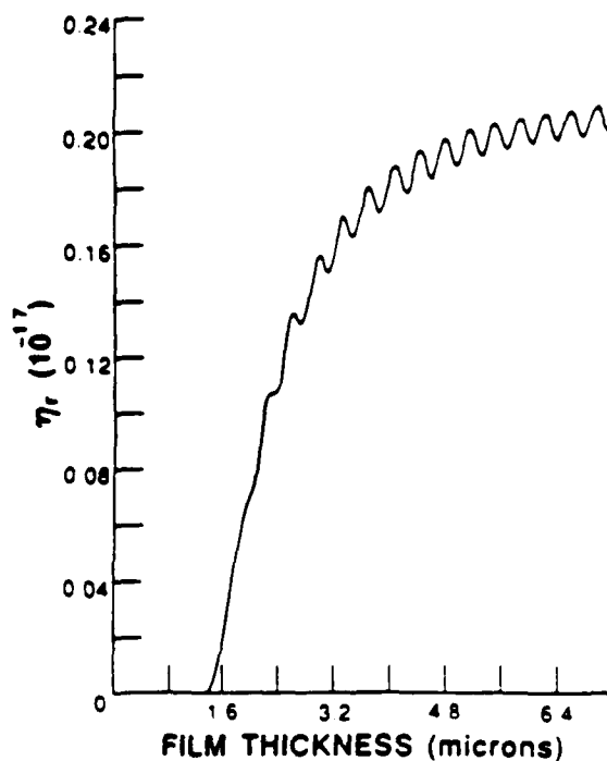
Fig. 5. The reflection ( \eta_r ) DFWM cross section versus film thickness for \theta_c = 45^\circ . Here n_c = 1.0 , n_f = 1.6 , n_s = 1.59 , n_{2lf} = 1 \times 10^{-16} \text{ m}^2/\text{W} and n_{2ls} = 0.0
