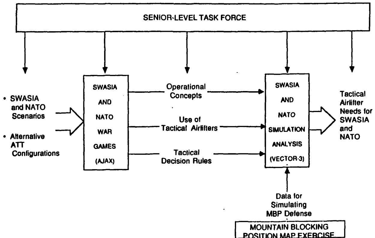
Figure 12-2. Study Methodology.
