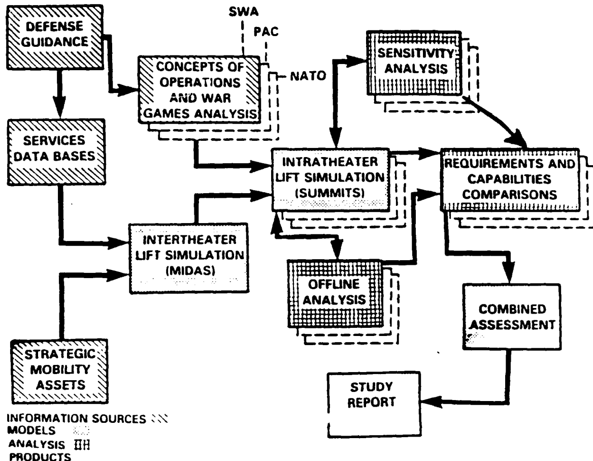
Figure 3-3. WIMS Methodology.
