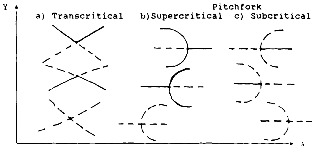
Figure 2-2 Simple Bifurcations
