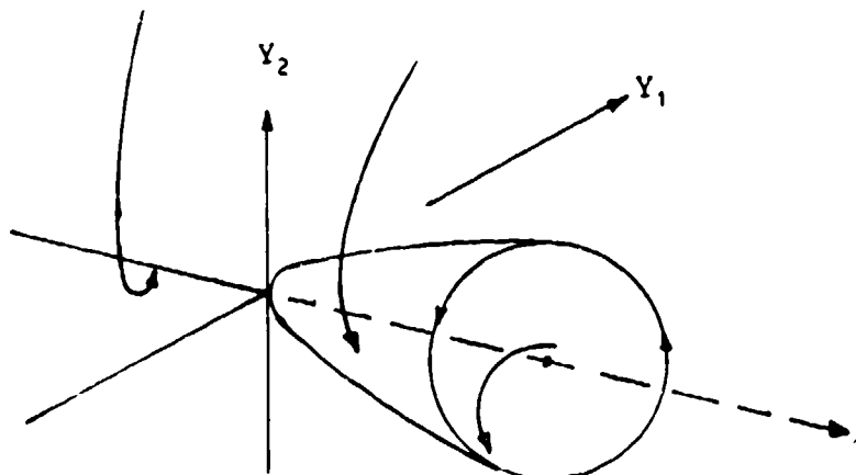
Figure 2-6 Hopf Bifurcation
