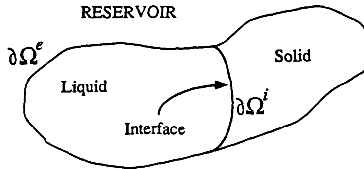
Figure 2.1: Physical problem with interior boundary
