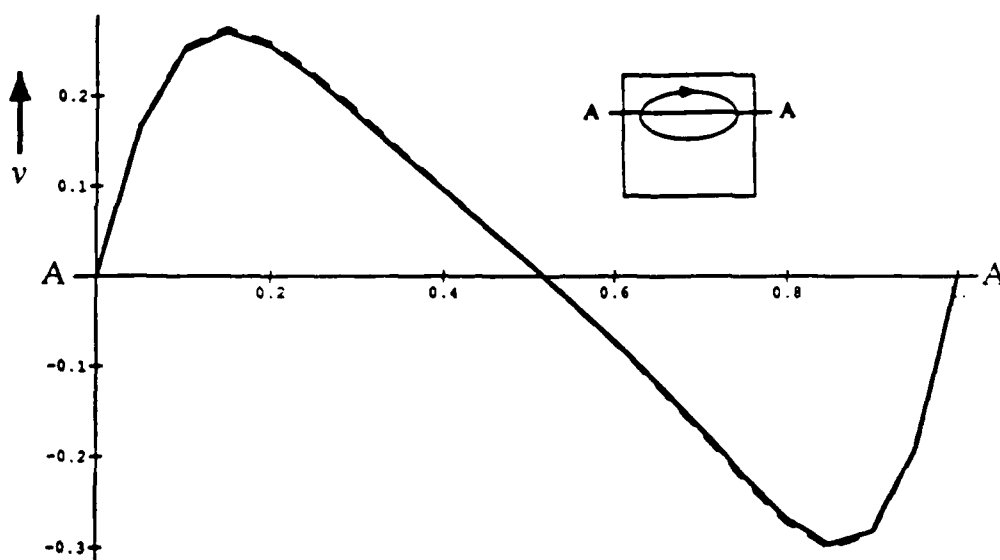
Figure 8.18: Vertical-velocity profile for high-order approximations
