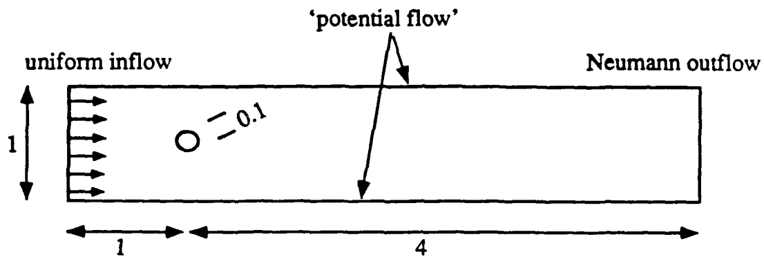
Figure 8.23: Physical domain and boundary conditions for cylinder in crossflow
