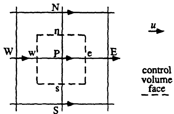
Figure 7.11: Diagram of variable locations for discrete u -momentum equation
