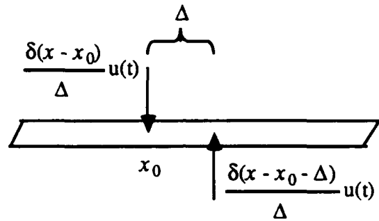
Figure 5-2. Point Moment
