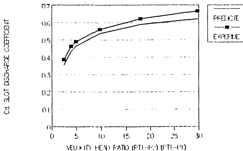
Figure 7.15: Predicted versus experimental values of C_d for the slot.
