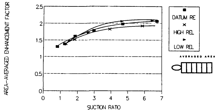
Figure 5.23: Effect of varying the duct Reynolds number ( Re_L ) on \overline{EF} for the 30^\circ hole. Datum Re_L = 25,000 ; high Re_L = 31,000 ; low Re_L = 13,000 .
