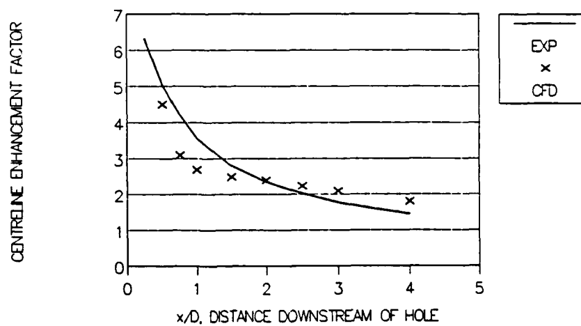
Figure 8.5: Heat transfer results for SR = 8 .
