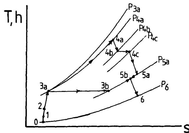
Figure 2.7: Model 2- coolant flow is added back to the core flow downstream of the rotor.
