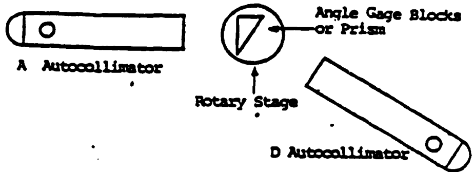
FIG. 2 Top View
