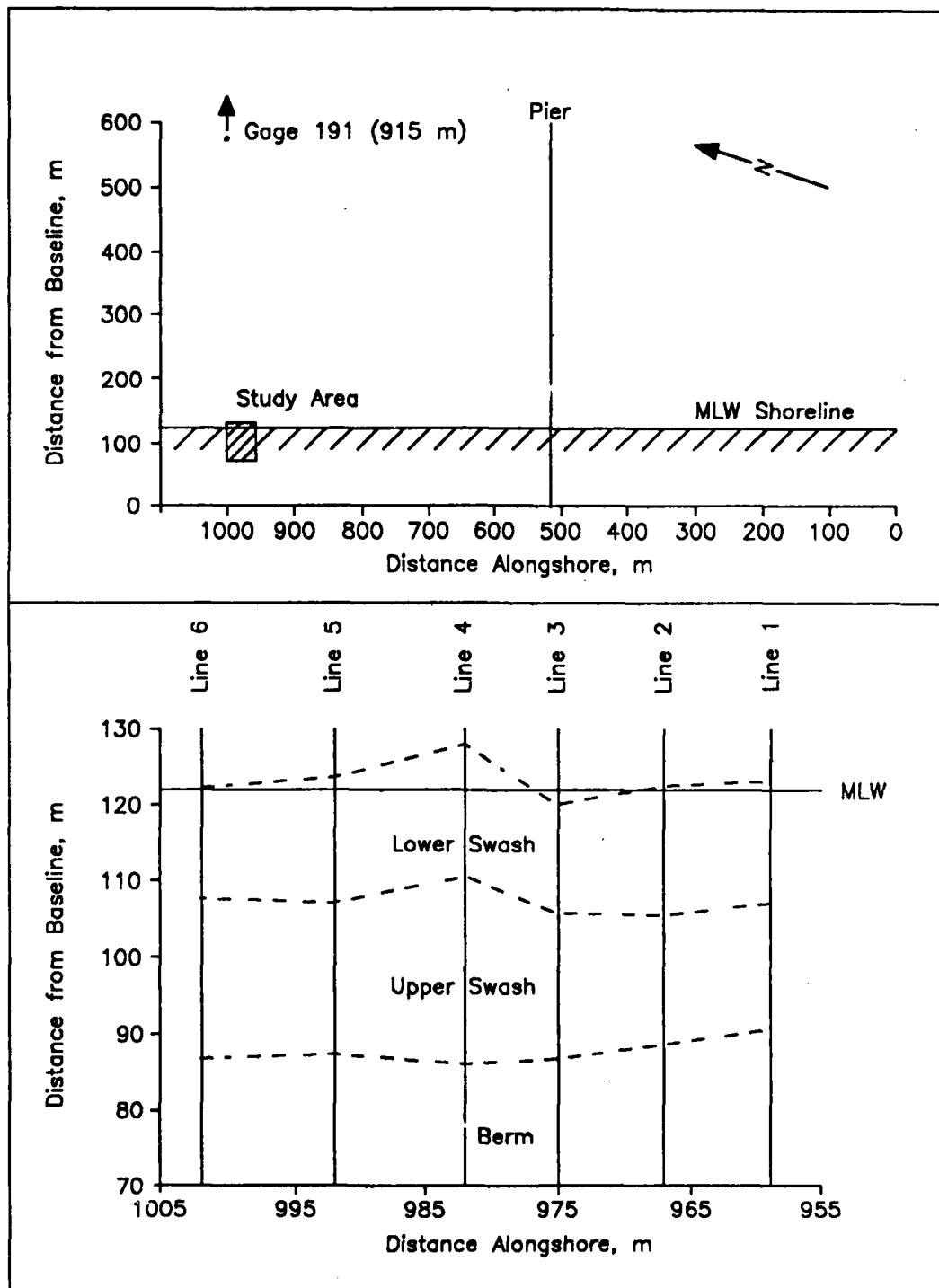
Figure 2. Schematic showing relative positions of transect lines and morphologic zones in the study area
