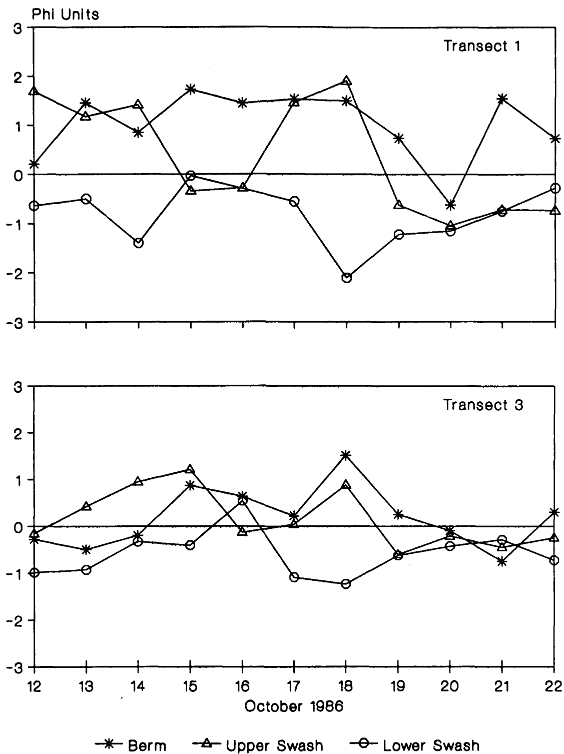
Figure 6. Comparison of trends in median grain size for berm, upper swash, and lower swash morphologic zones (Continued)
