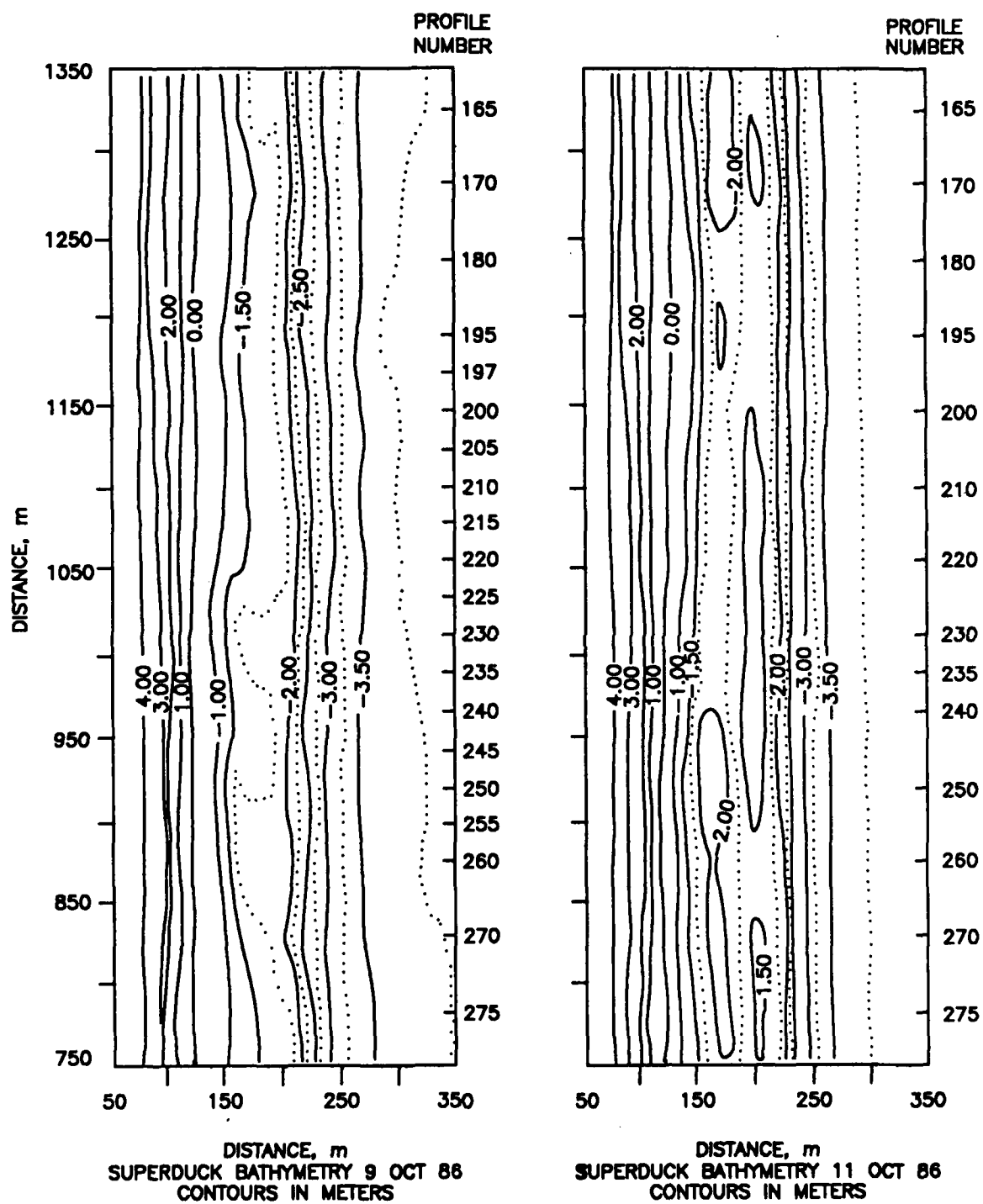
Figure 4. Contour maps of bathymetry for 9 and 11 October 1986 showing the positions of surveyed profile lines
