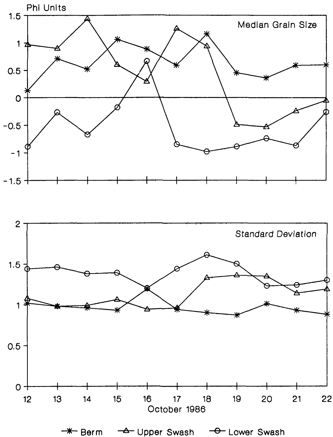
Figure 8. Plot of average median grain size and standard deviation for berm, upper swash, and lower swash zones
