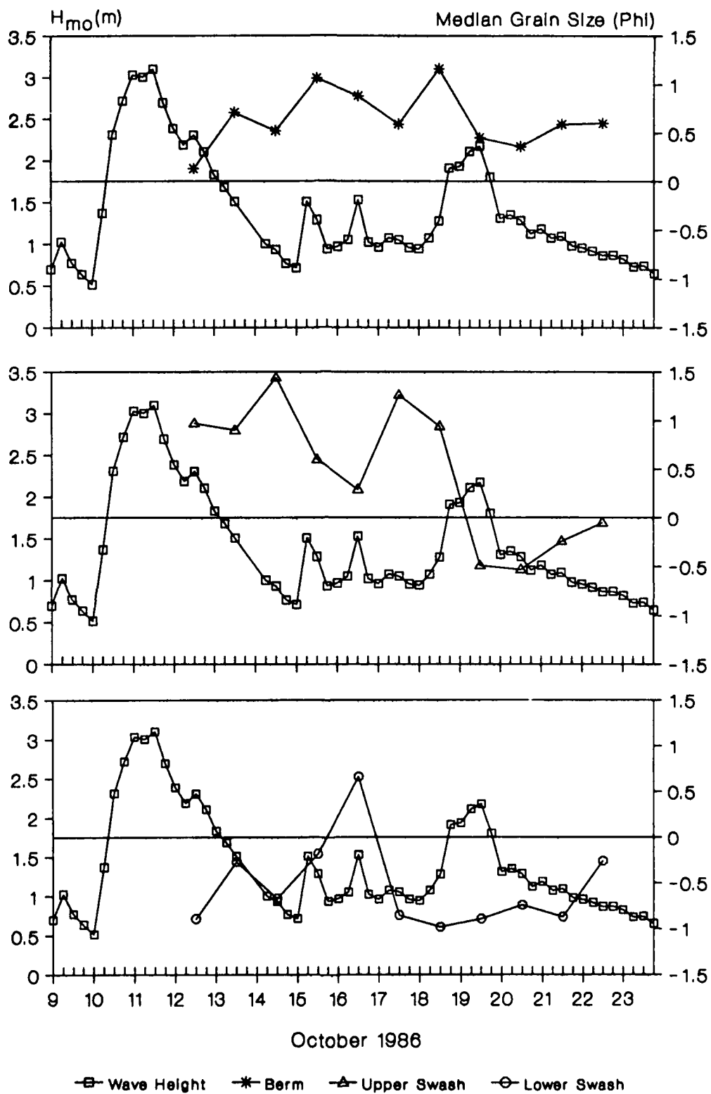
Figure 7. Comparison of trends in median grain size and wave height for berm, upper swash, and lower swash zones
