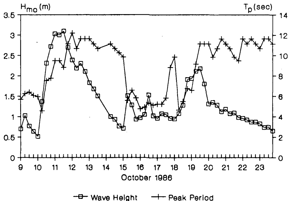
Figure 3. Plot of wave height and period measured at gage 191
