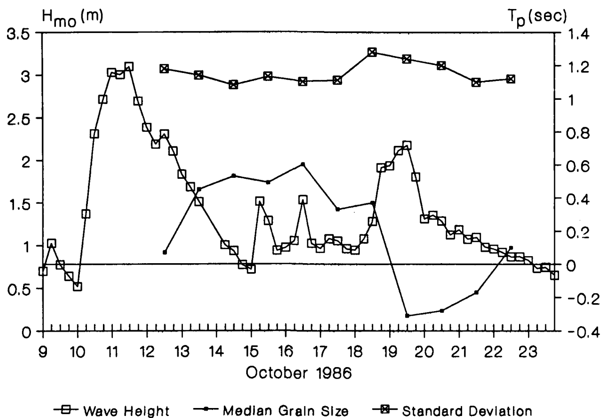
Figure 9. Plot of wave height, average median grain size, and average standard deviation for 9 to 23 October 1986
