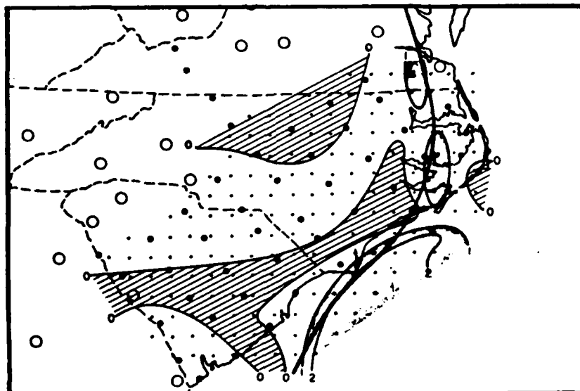
Figure 4.1a - Local frontogenesis at 1200 UTC 25 January 1986. Negative regions are represented by hatched areas. Values greater than 1°K/100 km/hour are shaded gray. The thick line is the frontal position from the surface analysis.
