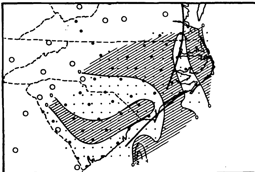
Figure 4.1h - Advection contribution at 1400 UTC 25 January 1986. Negative regions are represented by hatched areas. Values greater than 1^{\circ}\text{K}/100\text{ km/hour} are shaded gray. The thick line is the frontal position from the surface analysis.
