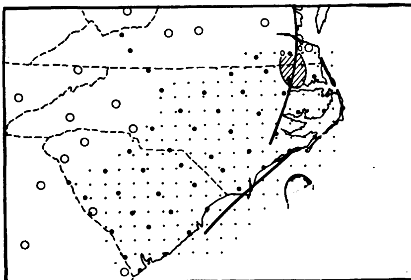
Figure 4.1i - Shear deformation at 1400 UTC 25 January 1986. Negative regions are represented by hatched areas. Values greater than 1^{\circ}\text{K}/100\text{ km/hour} are shaded gray. The thick line is the frontal position from the surface analysis.
