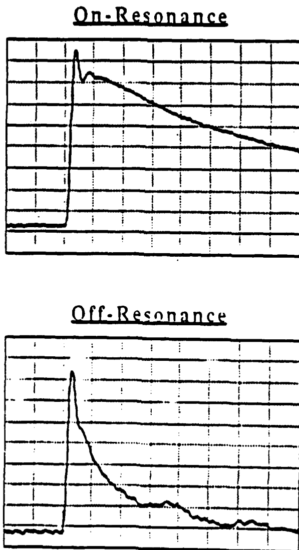
Figure 1: Changes in the absorption of the diode laser probe beam are shown following 193 nm photolysis of \text{I}_2 in a 1/10 mixture with \text{CO}_2 at a total pressure of 27.5 mTorr. The diode laser monitors the 00^0_1, J=13 \rightarrow 00^0_2, J=12 ro-vibrational transition of \text{CO}_2 in the upper trace. The diode laser is tuned off the absorption line in the lower trace. Each trace is 20 \mu\text{s} full scale. The vertical axes are not scaled relative to one another.
