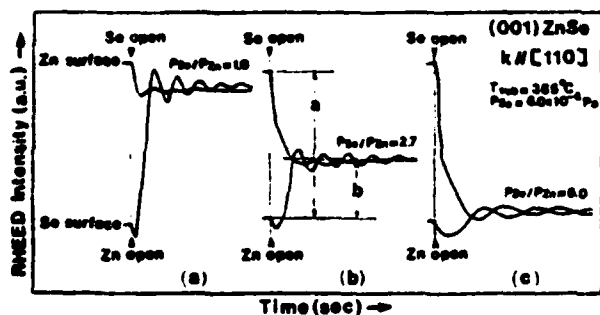
Fig. 3 The dependence of RHEED intensity oscillation on growth condition.
