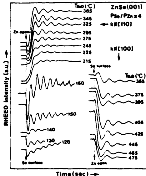
Fig. 2 RHEED intensity oscillations during MBE growth of ZnSe at various substrate temperatures. The Se-to-Zn pressure ratio is 4.
