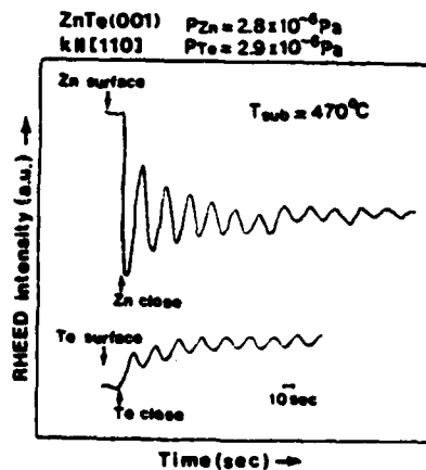
Fig. 4 RHEED intensity oscillation behaviors during sublimation of ZnTe at the substrate temperature of 470°C, initiated from Zn- and Te- covered surfaces respectively.
