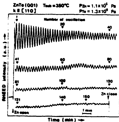
Fig. 1 RHEED intensity oscillations during MBE growth of ZnTe on ZnTe predeposited layer on GaAs (001) with k [110]. The growth is initiated by impinging Zn flux on the Te-covered surface. The substrate temperature is 350°C, and the Te-to-Zn pressure ratio is 1.
