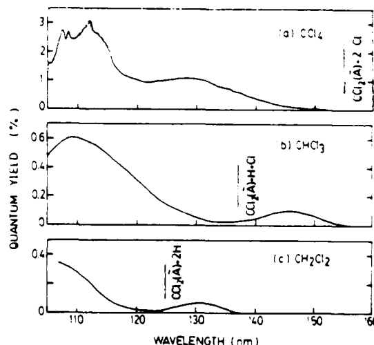
Fig. 2. Fluorescence quantum yields of (a) \text{CCl}_4 , (b) \text{CHCl}_3 , and (c) \text{CH}_2\text{Cl}_2 . The calculated thresholds for the dissociation processes that produce \text{CCl}_2(\tilde{\text{A}}-\tilde{\text{X}}) fluorescence are indicated.
