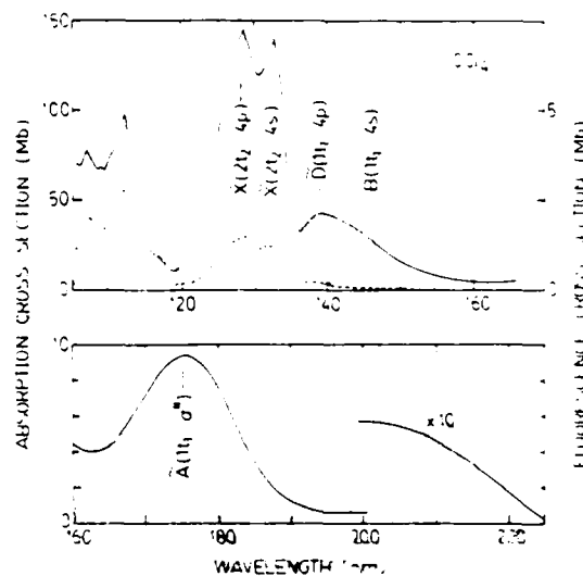
Fig. 1. Photoabsorption (—) and fluorescence (---) cross sections of \text{CCl}_4 measured with a monochromator resolution of 0.2 nm.
