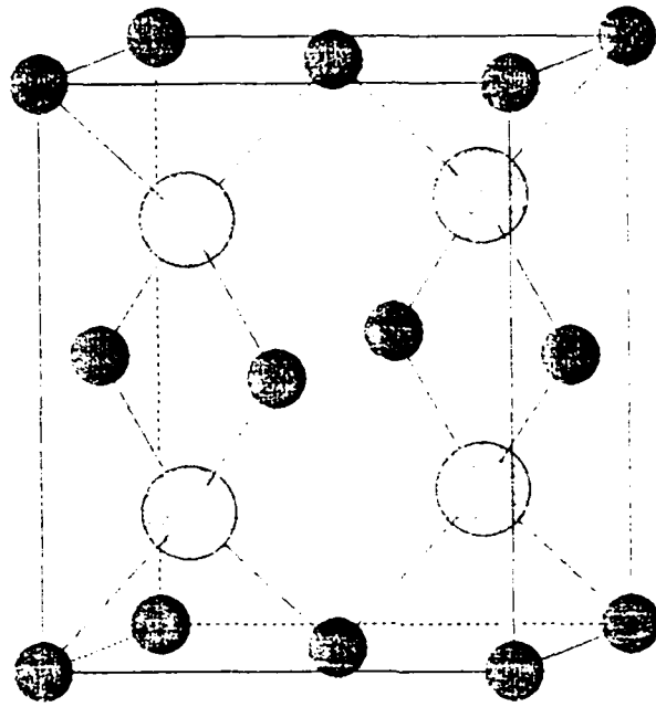
● Palladium ○ Oxygen
