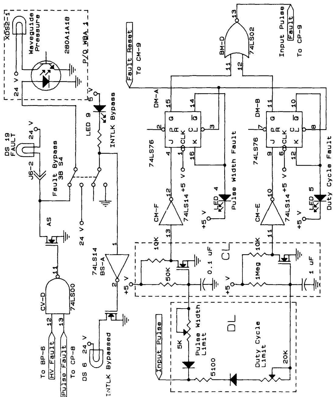
Fig. 4-12. Pulse Fault Detector and Fault Summary
