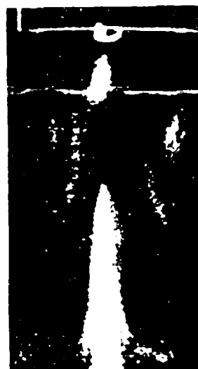
Figure 8. Pattern of the fluid motion at low Reynolds numbers ( R \approx 30 ) in the x, z -plane.
