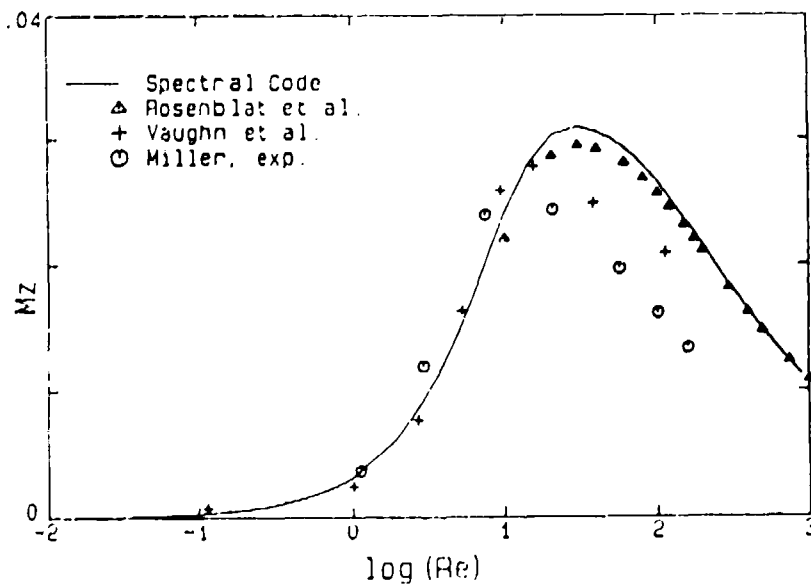
Figure 9. Roll moment M_z vs Reynolds number Re for \eta = 4.368 , \tau = 0.16667 , and \theta = 20^\circ . Comparison with numerical and experimental data.
