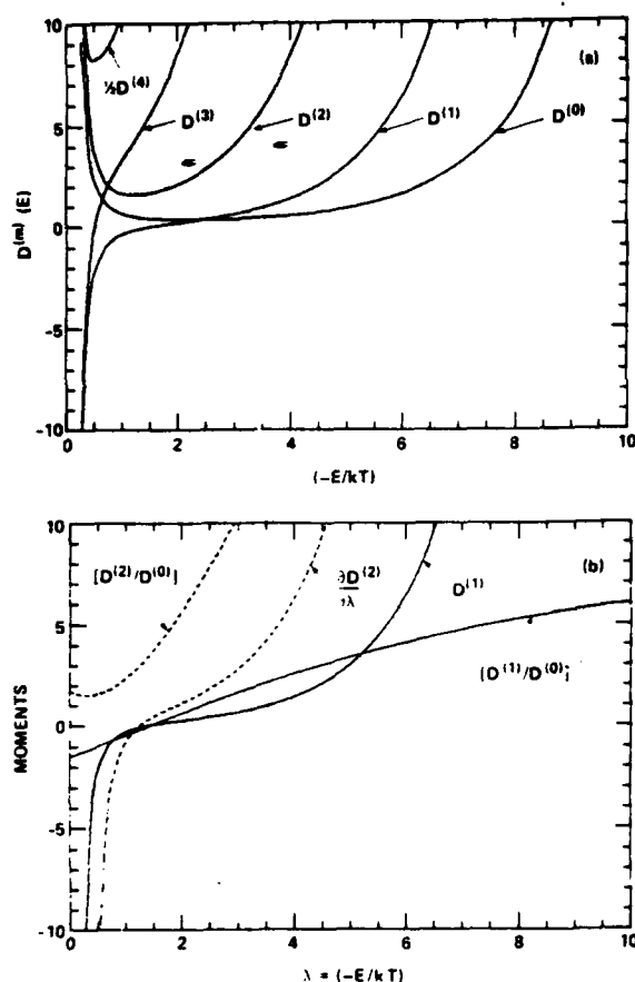
FIG. 1. (a) Normalized moments D^{(m)} of energy change rate (energy s^{-1} ), m = 0-4 , as a function of internal energy E_i = -\lambda(kT) of the bound ion pair. (b) Averaged energy change and energy-change squared D^{(m)}/D^{(0)} per collision, D^{(1)} and derivative of D^{(2)} . Equal-mass species and charge-transfer ion-neutral collisions are assumed and moments are normalized to the quantity (-1)^m \Gamma \alpha_T (kT)^{m-1} \bar{N}_A \bar{N}_B .
