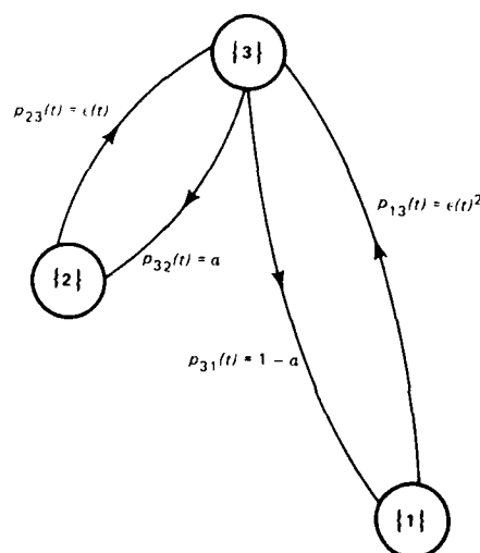
FIG. 5. The Markov process of Example 4.
