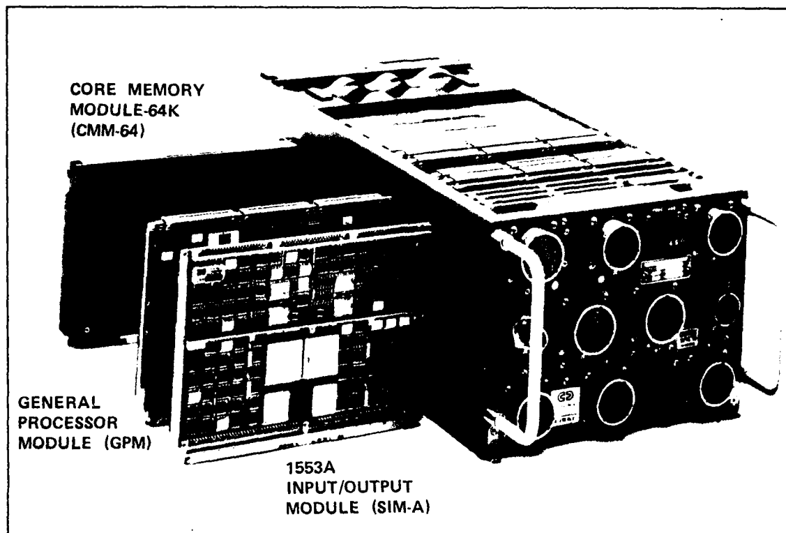
Fig. 4-3 AN/AYK-14 Computer
