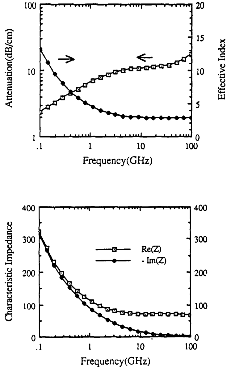
Fig. 5. 4. Transmission characteristics of section B
