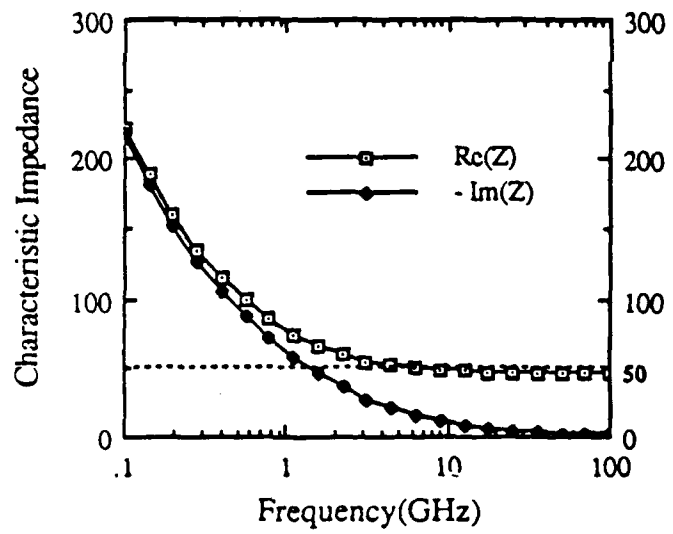
Fig. 5. 5. Transmission characteristics of the slow-wave electrode
