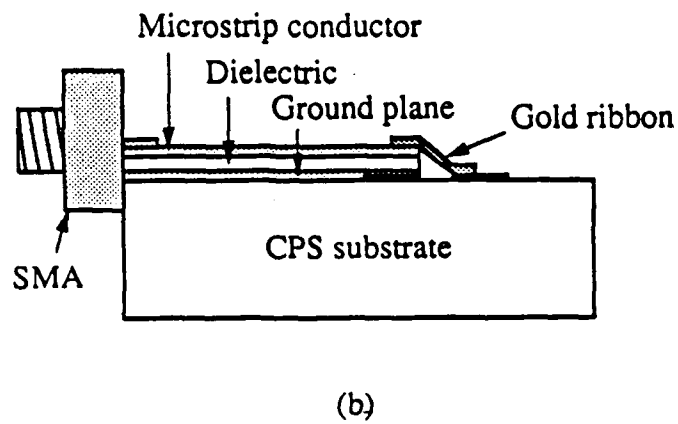
Fig. 4. 1. Schematic diagram of the coplanar strip feed:
