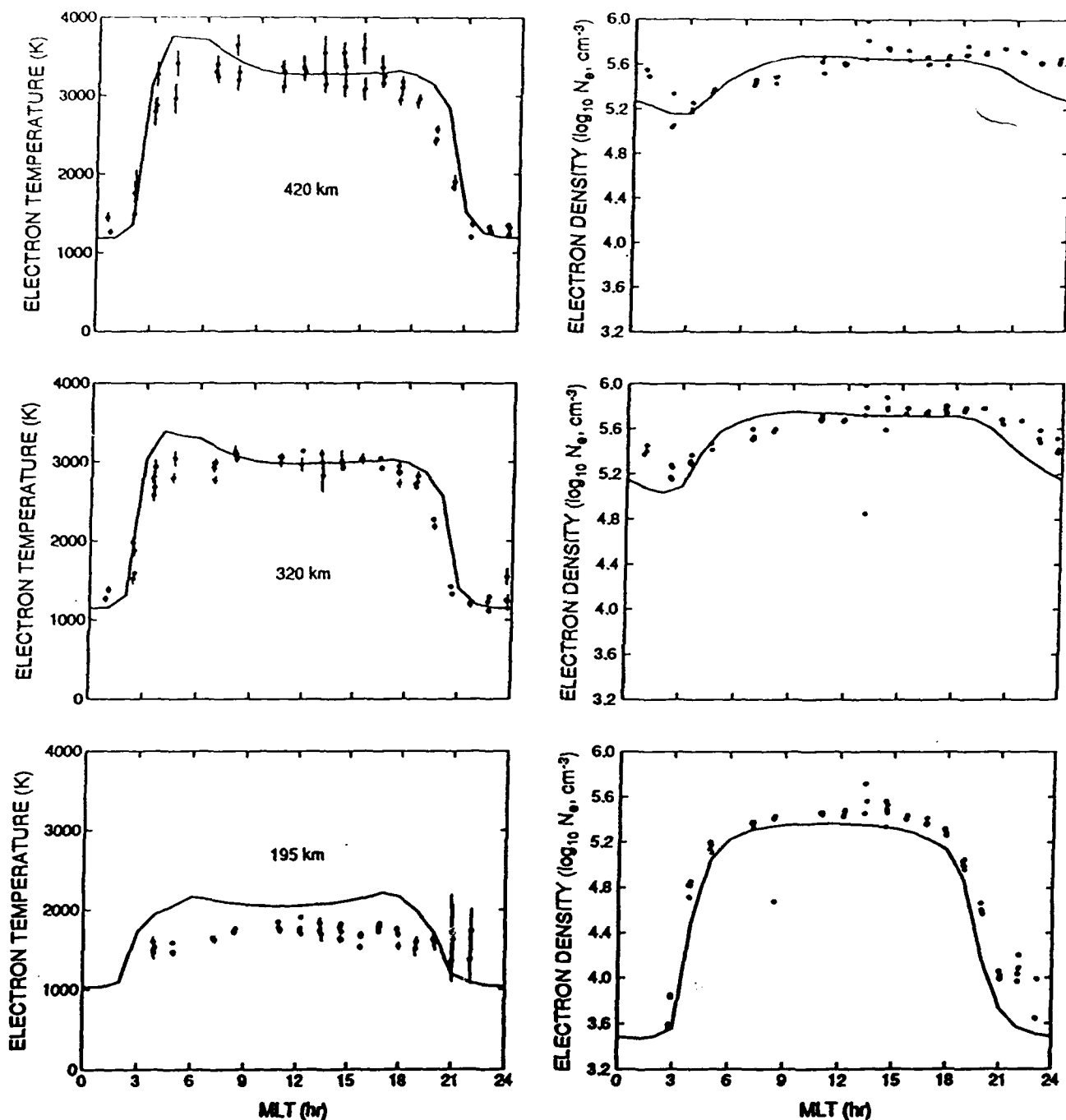
Figure 3. Comparison of the model electron density and temperature predictions with Millstone Hill measurements at 55^\circ (\pm 1^\circ) and at three different altitudes: 420 km (top panel); 320 km (middle panel); and 195 km (bottom panel). Electron temperatures are compared in the left column, and electron densities in the right. The model results are plotted as a solid line, and the radar measurements are plotted as solid circles. From Paper 12.
