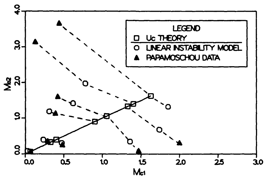
Figure 2.25 Plot of M_{c1} versus M_{c2} showing a comparison between the theoretical U_c from equation (1.2), the linear stability prediction (the phase speed of the neutral mode), and the experimental data from Papamoschou [1989].
