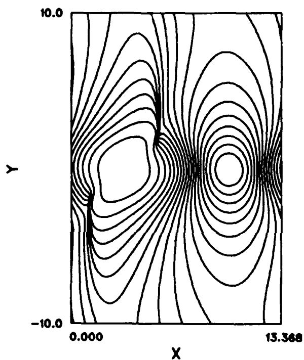
Figure 4.39 Embedded shock waves (a) pressure contours, (b) Mach contours M = \sqrt{u^2 + v^2}/c .
