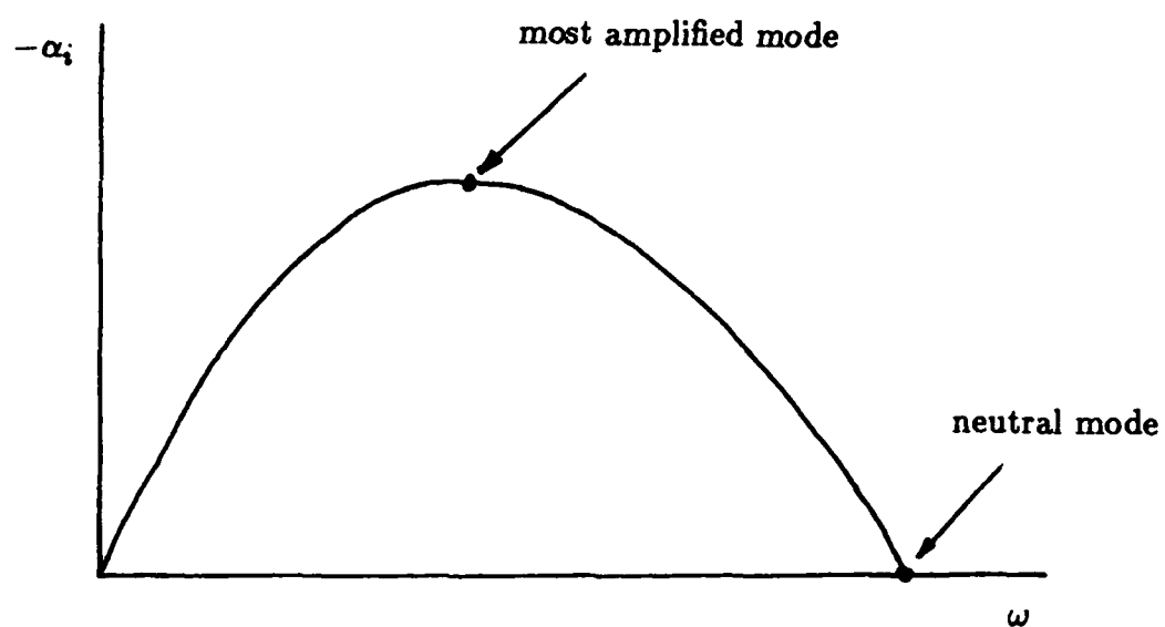
Figure 2.24 Amplification rate versus frequency, defining the most amplified wave, and the neutral wave.
