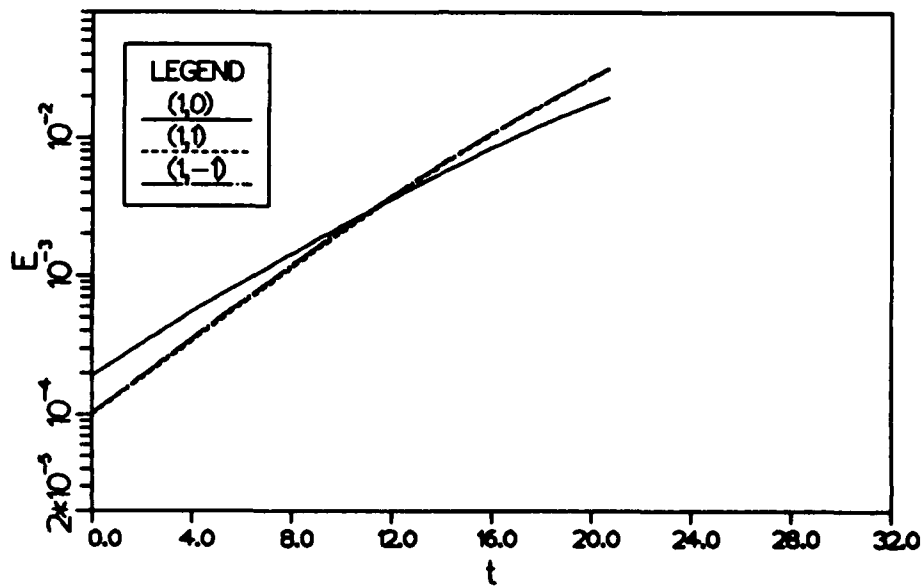
Figure 5.52 Growth in mode energies of the unstable waves in the presence of background noise.
