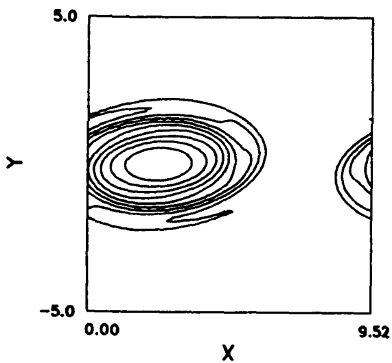
Figure 4.28 Developed structure at M_1 = 0.6 (a) temperature, (b) stagnation enthalpy, (c) entropy.
