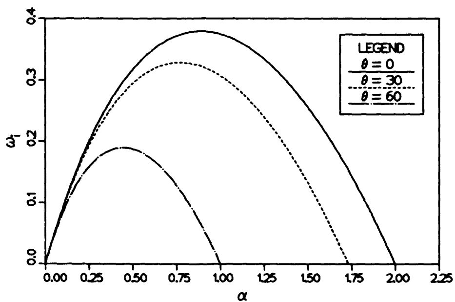
Figure 2.7 Temporal amplification rate of oblique waves at M_1 = 0.01
