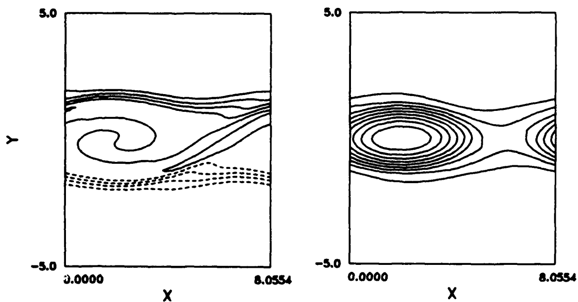
Figure 4.7 Structure at long time (a) mixture fraction, (b) vorticity.
