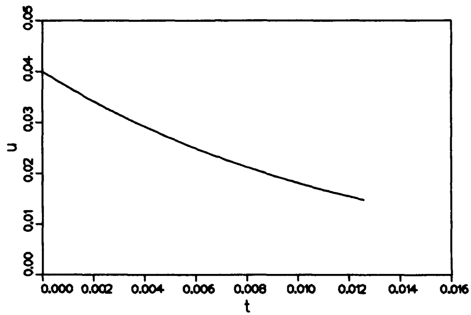
Figure 3.1 Decay of u velocity at x = 0.5 z = 0.25 , for Taylor-Green problem.
