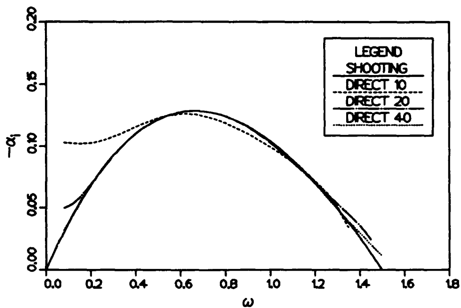
Figure A.1 Illustration of the convergence of the direct method. The number of points used ( N^* ) is given in the legend. The correct solution, as found by the shooting method, is also shown.
