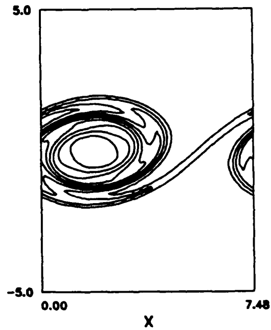
Figure 4.10 Developed structure at M_1 = 0.2 (a) mixture fraction, (b) pressure, (c) \omega_z , (d) \omega_z/\rho .
