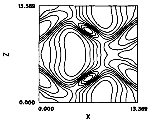
Figure 5.33 Cuts at y = 0 through the final structure developed at M_1 = 0.8 (a) mixture fraction (b) pressure.
