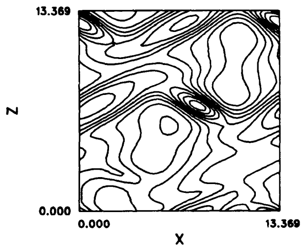
Figure 5.55 Simulation with random initial conditions at time t = 52.0 (a) carpet plot of mode energies, (b) pressure cut at y = 0 .
