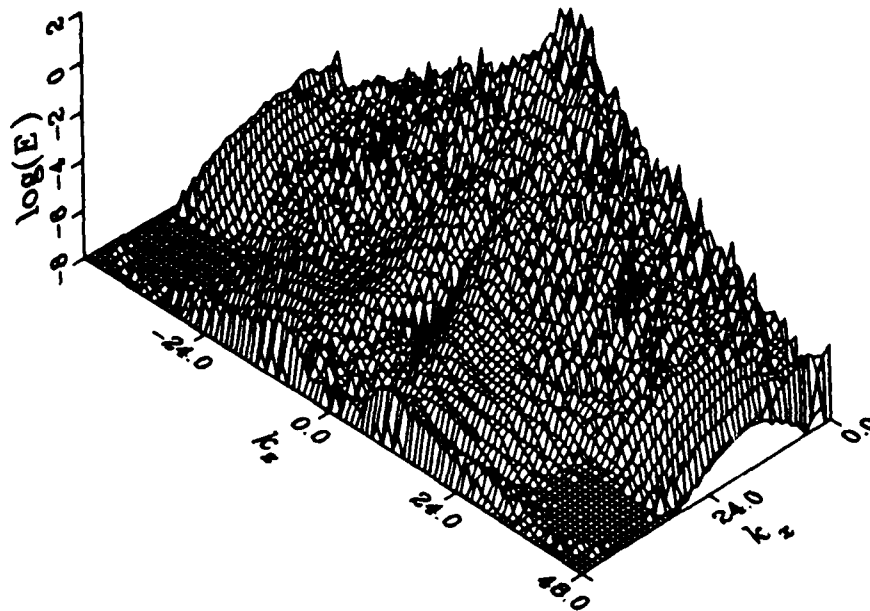
Figure 5.23 Carpet plot of the modal energy contents at the end of the three-dimensional simulation at M_1 = 0.8
