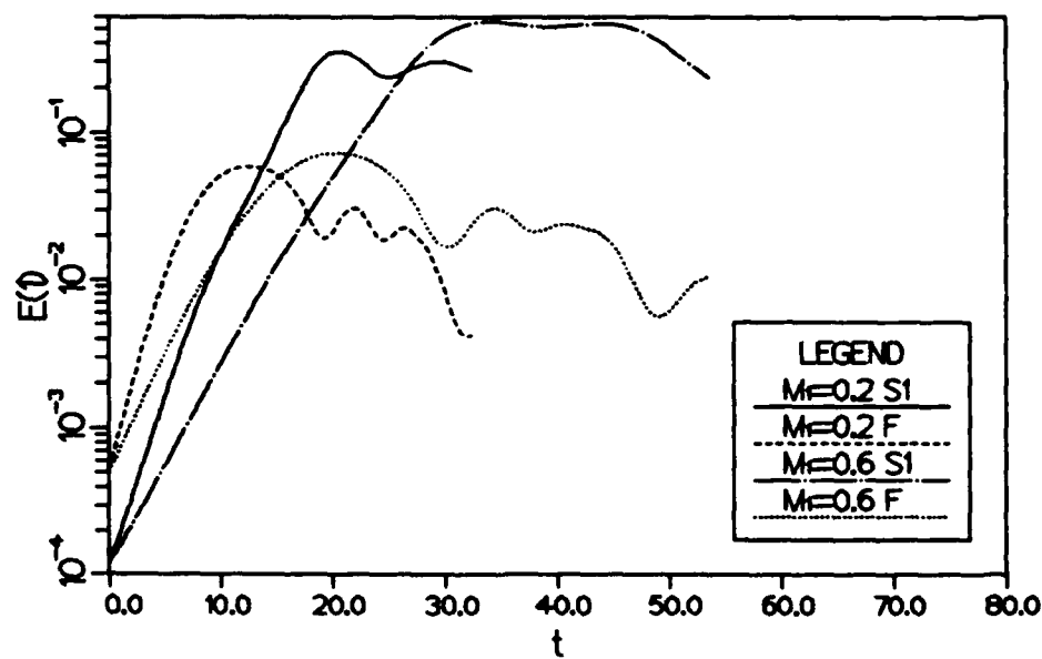
Figure 4.17 Growth in mode energy E , comparing M_1 = 0.2 with M_1 = 0.6 .
