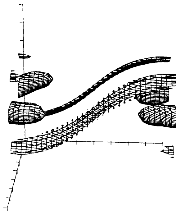
Figure 5.26 Perspective view of streamwise vorticity in the structure that developed at M_1 = 0.4
