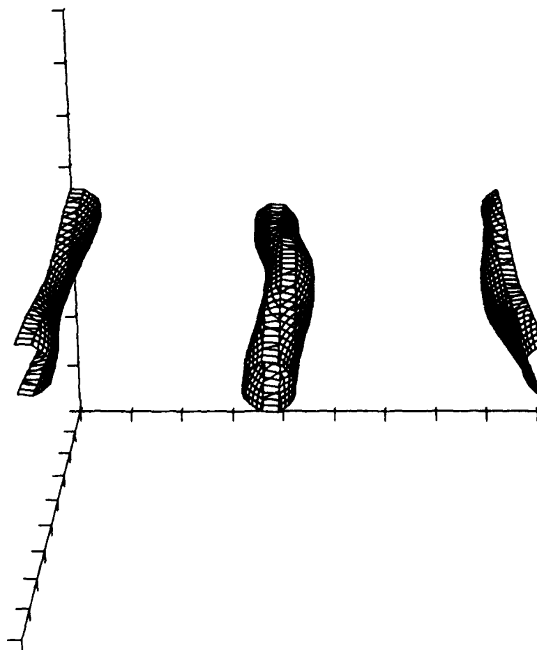
Figure 5.15 Perspective view of the pressure minima at time t = 12.63 for the helical subharmonic mode of instability, showing vortex cores at saturation on the fundamental instability.
