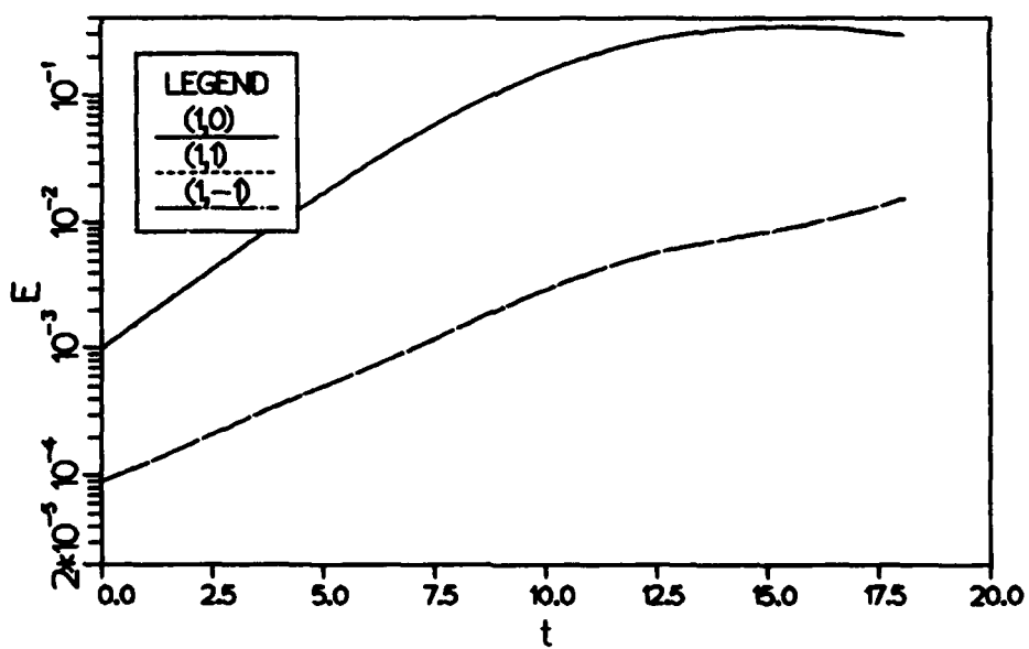
Figure 5.7 Growth in energy for the translative instability at M_1 = 0.4 . (1,0) is the two-dimensional wave. (1,1) and (1,-1) are the oblique waves.
