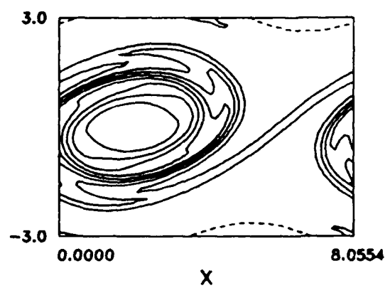
Figure 3.6 Developed structure for L_y = 6 (a) mixture fraction (b) vorticity.
