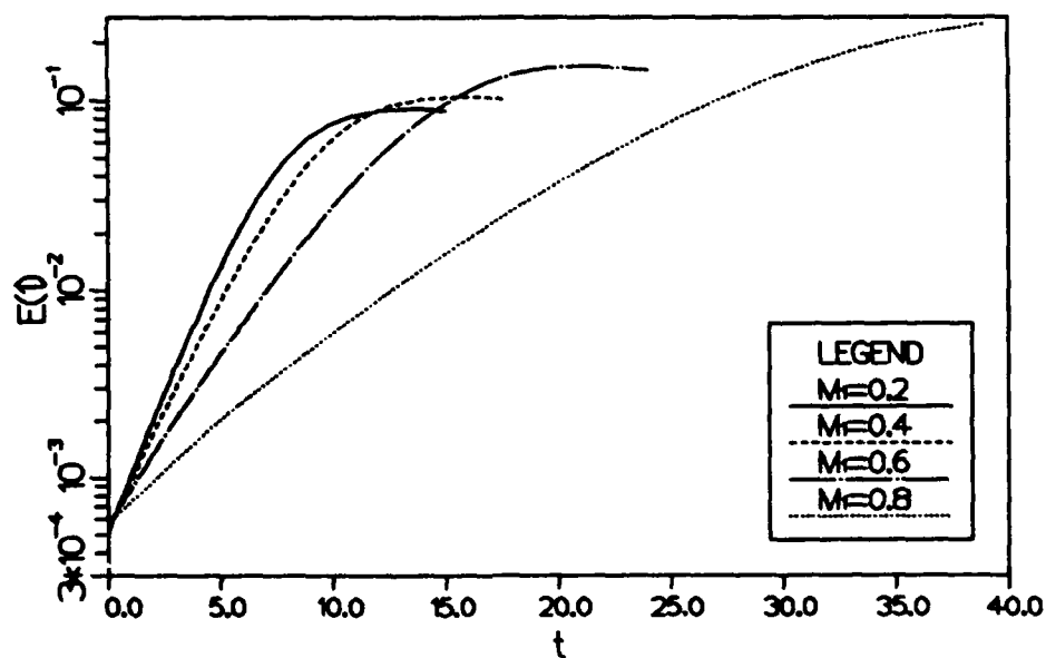
Figure 4.9 Effect of Mach number on the growth in mode energy E of the most amplified disturbance.
