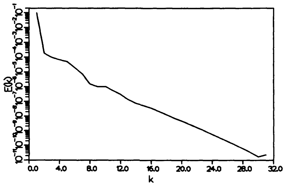
Figure 3.7 Energy spectrum for the case L_y = 10 , M_1 = 0.4 .
