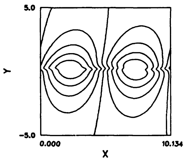
Figure 4.38 Convection of structure at T_2 = 5 shown by pressure contours (a) t = 0.0 , (b) t = 26.4 .
