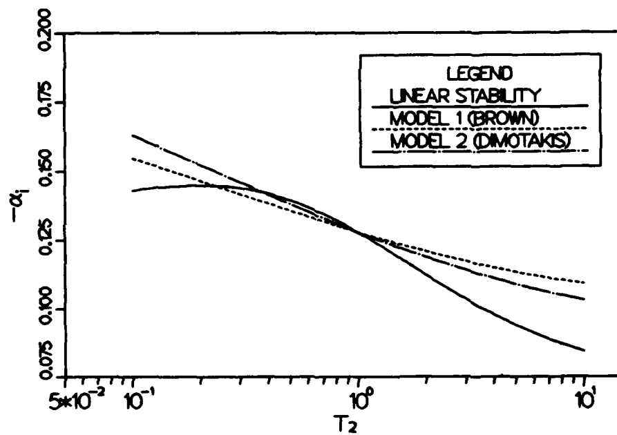
Figure 2.4 Variation in maximum spatial amplification rate with density ratio compared with models for growth rate from Brown [1974] and Dimotakis [1986], for velocity ratios: (a) U_2 = 0 , (b) U_2 = 0.5 .
