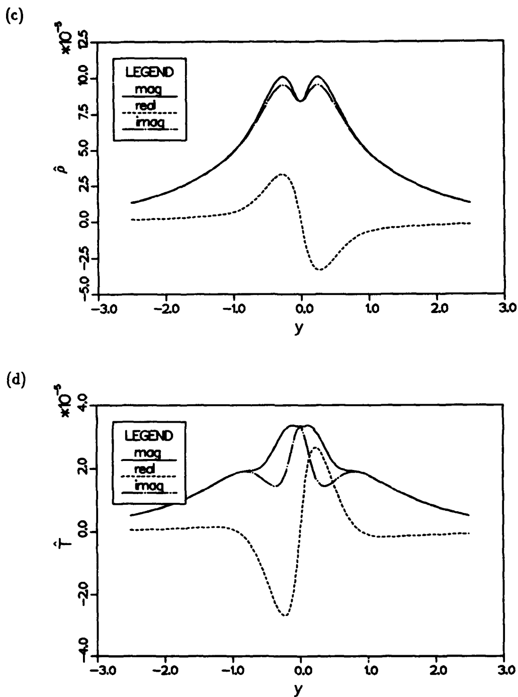
Figure 2.20 Eigenfunctions from temporal stability analysis at M_1 = 0.01 (a) \hat{u} , (b) \hat{v} , (c) \hat{\rho} , (d) \hat{T} .
