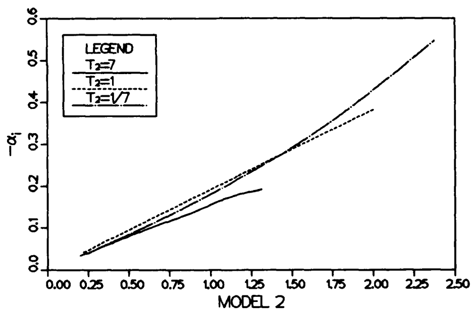
Figure 2.5 Plot of amplification rate against the functional form of the models of (a) Brown [1974] (model 1) and (b) Dimotakis [1986] (model 2).
