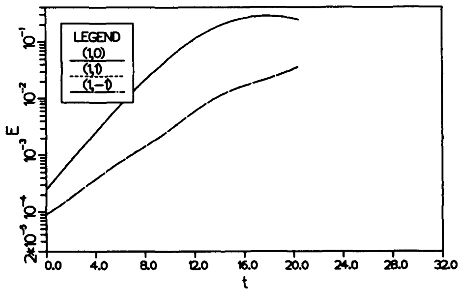
Figure 5.19 Growth in mode energies at M_1 = 0.4 (1,0) is the two-dimensional mode. (1,1) and (1,-1) are the oblique waves.
