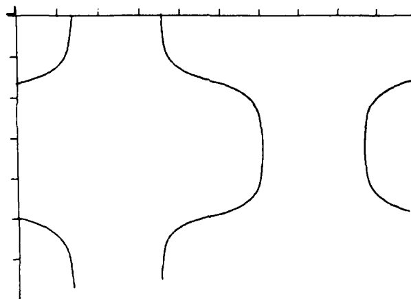
Figure 5.31 Vortex lines through the peaks of vorticity for the developed structure at M_1 = 1.05 (a) perspective view (b) top view.
