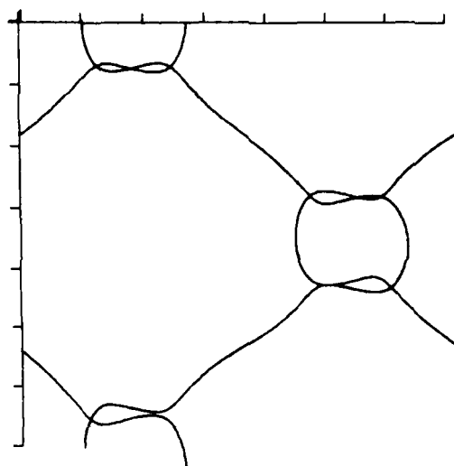
Figure 5.48 Vortex lines through structure developing from a pair of equal and opposite oblique waves.
