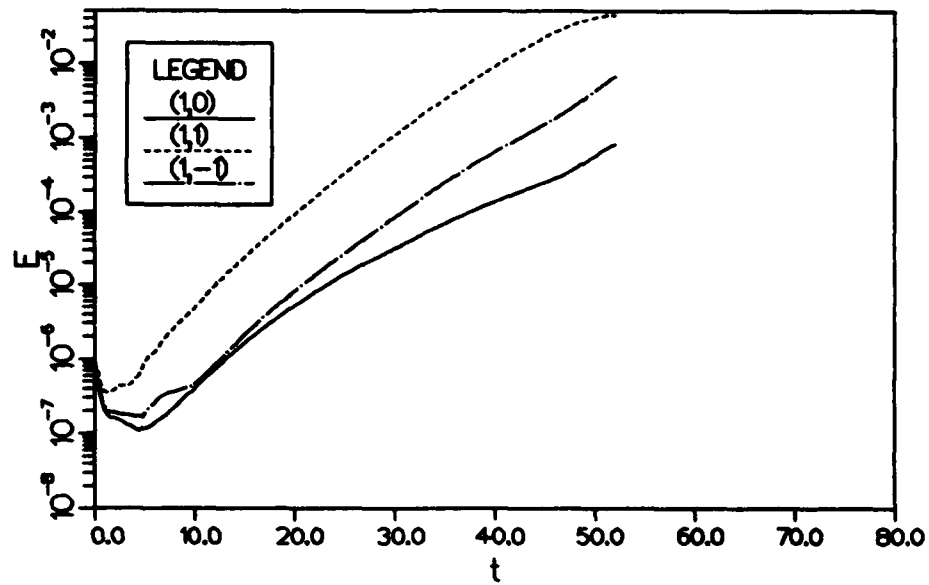
Figure 5.57 Growth in mode energies of the unstable waves in the simulation beginning with purely random initial conditions.
