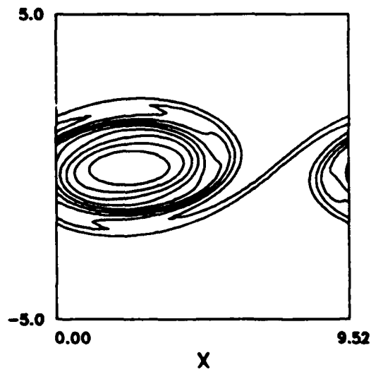
Figure 4.12 Developed structure at M_1 = 0.6 (a) mixture fraction, (b) pressure, (c) \omega_z , (d) \omega_z/\rho .
