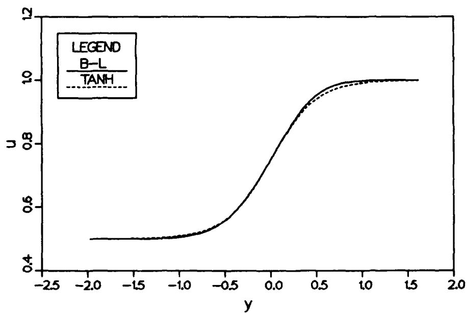
Figure 2.1 Comparison of velocity profile from solution of the boundary-layer equations with a hyperbolic tangent (a) U_2 = 0 , (b) U_2 = 0.5 .
