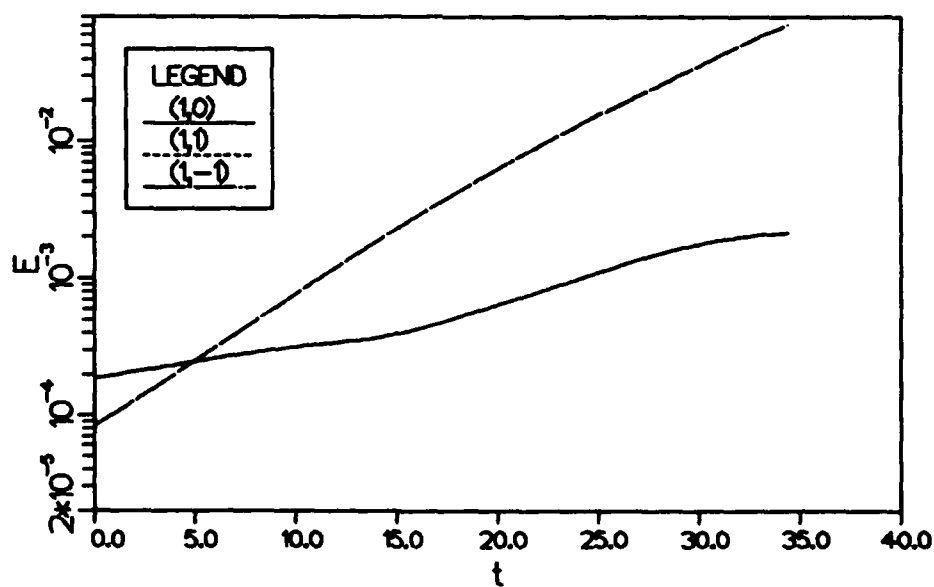
Figure 5.21 Growth in mode energies at M_1 = 1.05 (1,0) is the two-dimensional mode. (1,1) and (1,-1) are the oblique waves.
