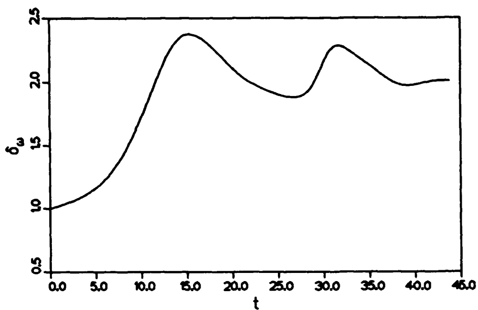
Figure 4.6 Long-time behavior of vorticity thickness at M_1 = 0.4 .
