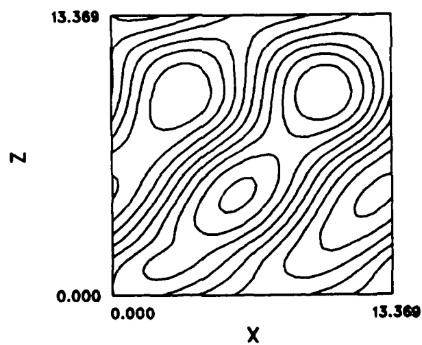
Figure 5.54 Simulation with random initial conditions at time t = 29.6 (a) carpet plot of mode energies, (b) pressure cut at y = 0 .
