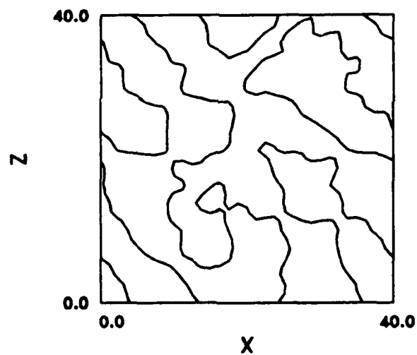
Figure 5.43 Flowfield at the end of the linear stage of instability growth at M_1 = 0.8 , shown by the v = 0 contour.
