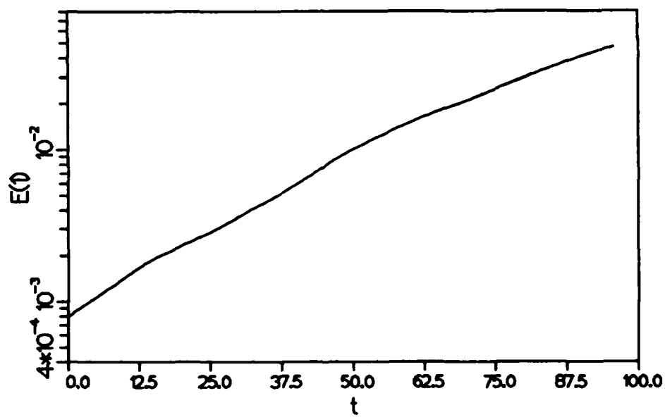
Figure 4.42 Growth of mode energy for supersonic instability mode.
