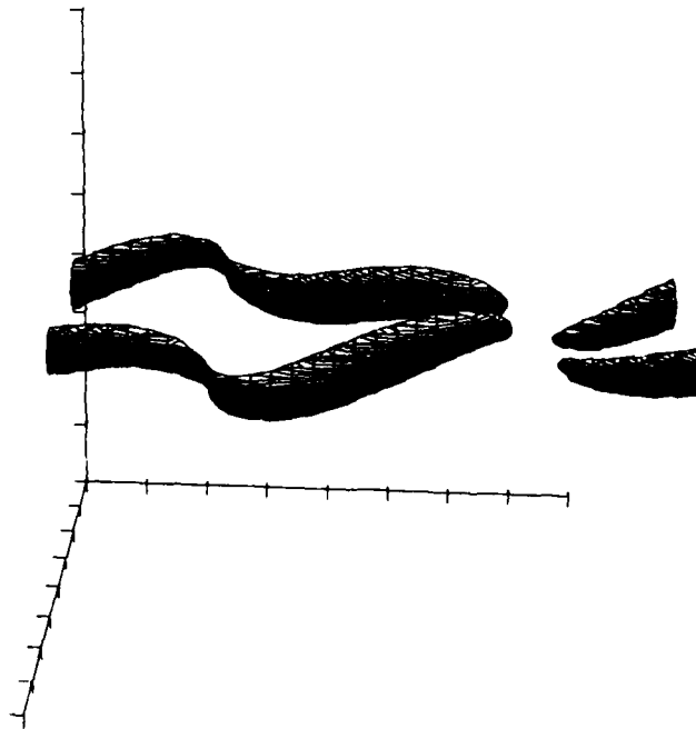
Figure 5.28 Surface of constant pressure showing the rotational region in the structure developing at M_1 = 1.05 .
