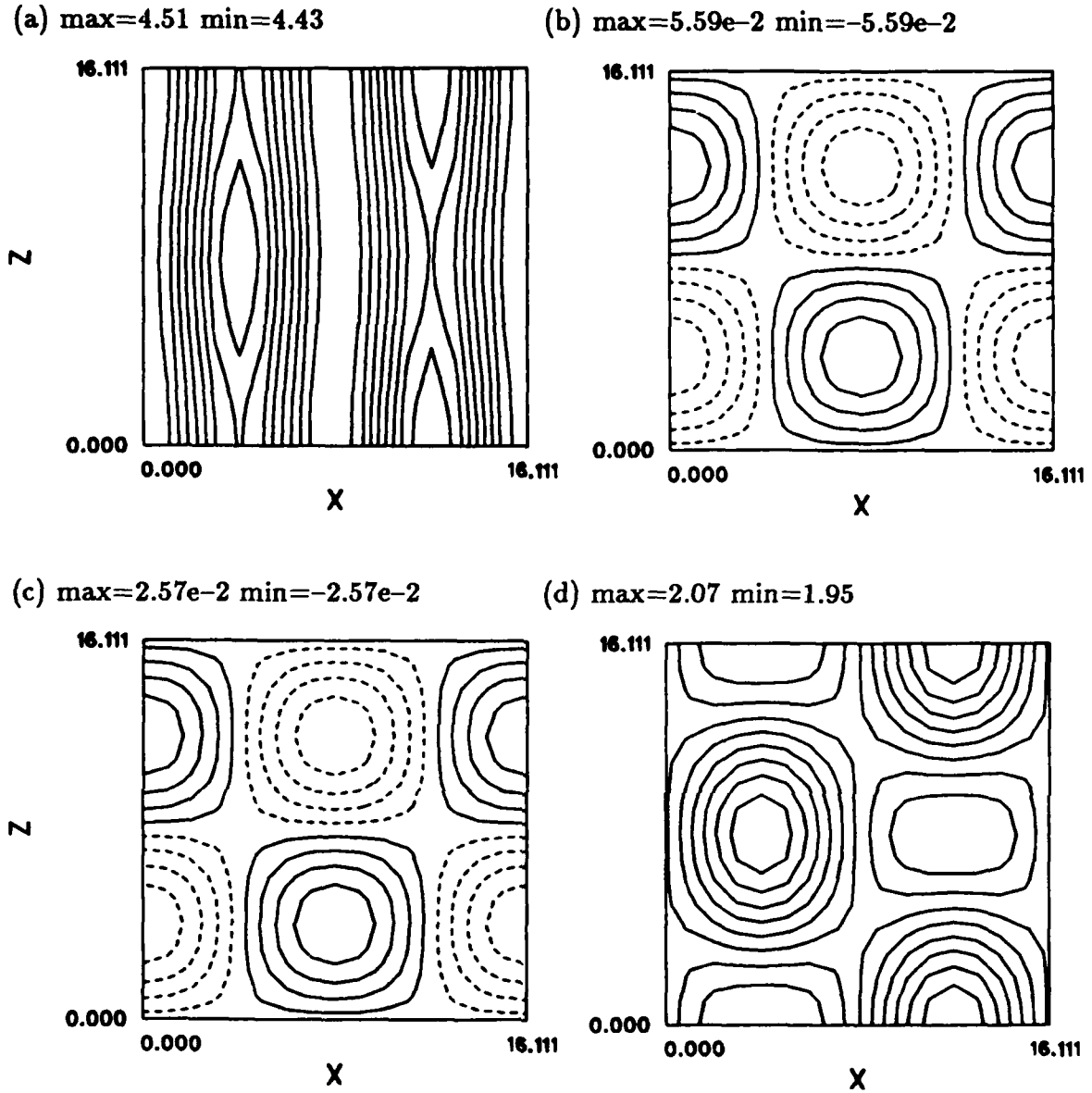
Figure 5.12 Initial condition for the 'helical' subharmonic mode of instability at M_1 = 0.4 (a) pressure - minimum at x = 0 , Lx/2 , maximum at L_x/4 , 3L_x/4 (b) \omega_x (c) \omega_y (d) \omega_z .
