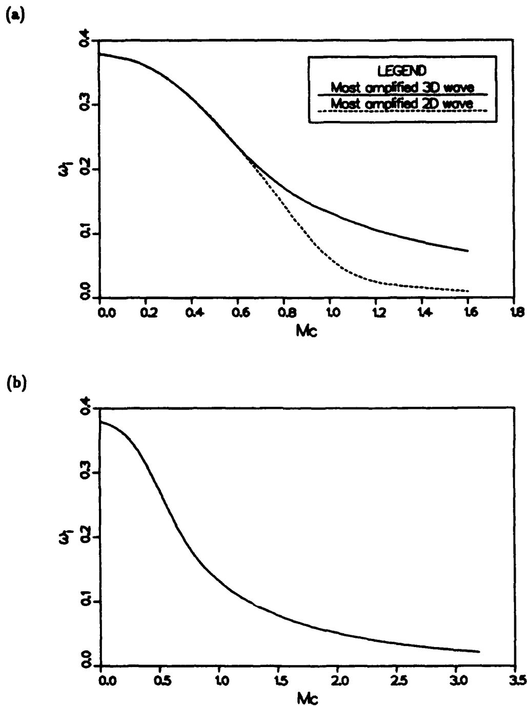
Figure 2.12 Variation of the amplification rate of the most unstable wave with Mach number, (a) comparing the most amplified wave with the most amplified two-dimensional wave, (b) extension to M_c = 3.2 for the most unstable wave.
