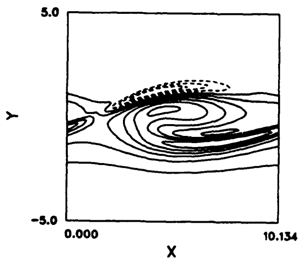
Figure 4.37 Developed structure at M_1 = 0.6 , T_2 = 5 (a) mixture fraction, (b) pressure, (c) \omega_z , (d) \omega_z/\rho .
