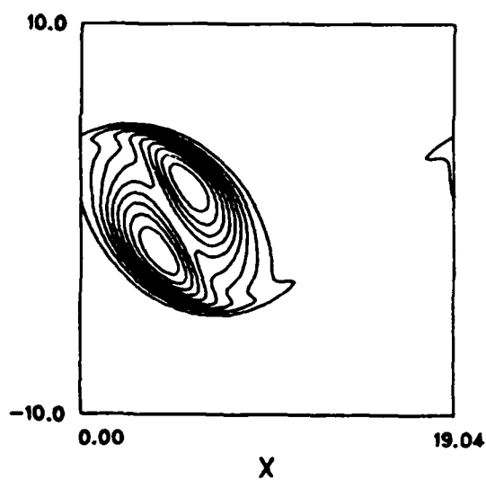
Figure 4.25 Step 3 in pairing process at M_1 = 0.6 (a) mixture fraction, (b) pressure, (c) \omega_z , (d) \omega_z/\rho .
