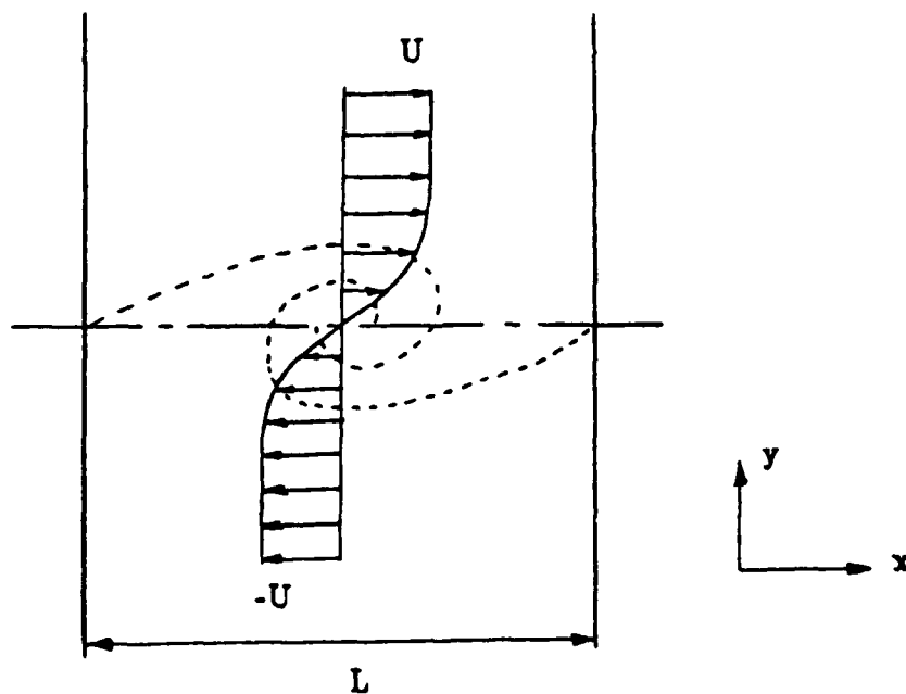
Figure 1.2 Time-developing mixing layer.
