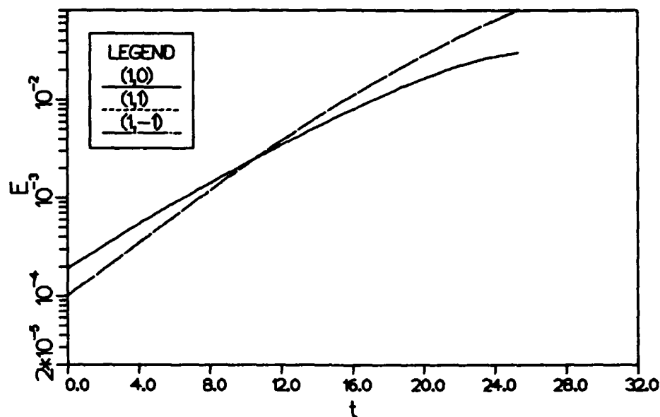
Figure 5.20 Growth in mode energies at M_1 = 0.8 (1,0) is the two-dimensional mode. (1,1) and (1,-1) are the oblique waves.
