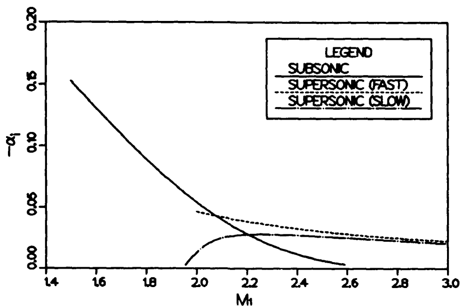
Figure 2.15 Variation in amplification rate with Mach number M_1 for the subsonic mode, the 'fast' supersonic mode, and the 'slow' supersonic mode.
