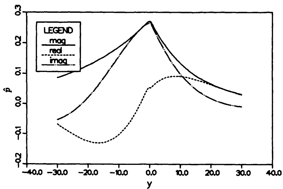
Figure 2.19 Eigenfunctions of pressure at M_1 = 2.2 for (a) the fast supersonic mode, (b) the slow supersonic modes and (c) the subsonic mode.
