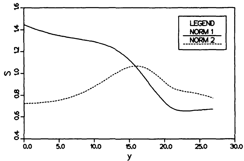
Figure 4.32 Time history of the peak strain rate. Non-dimensionalized as S = S^* \delta_0^* / U_1^* (norm 1), or as S = S^* \delta^* / U_1^* (norm 2).
