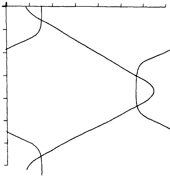
Figure 5.30 Vortex lines through the peaks of vorticity for the developed structure at M_1 = 0.8 (a) perspective view (b) top view.
