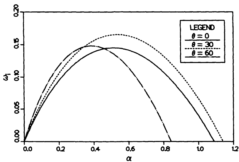
Figure 2.8 Temporal amplification rate of oblique waves at M_1 = 0.8
