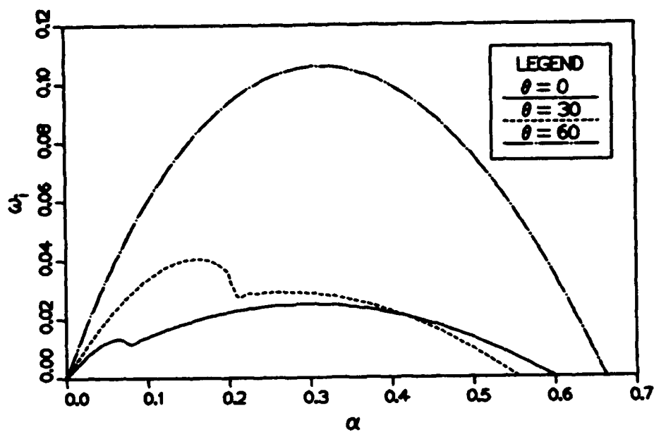
Figure 2.9 Temporal amplification rate of oblique waves at M_1 = 1.2
