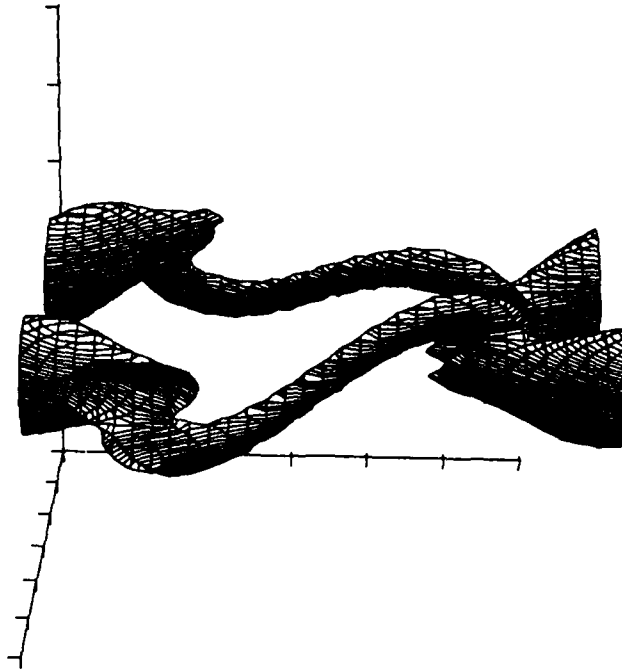
Figure 5.27 Surface of constant pressure showing the rotational region in the structure developing at M_1 = 0.8 .
