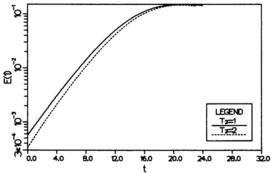
Figure 4.34 Growth in mode energy E , for temperature ratios 1 and 2.
