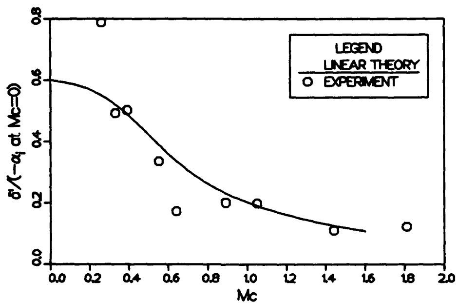
Figure 2.14 Growth rate data from Papamoschou [1986] normalized by the amplification rate of the most unstable wave, for the given velocity and density ratio, at zero Mach number
