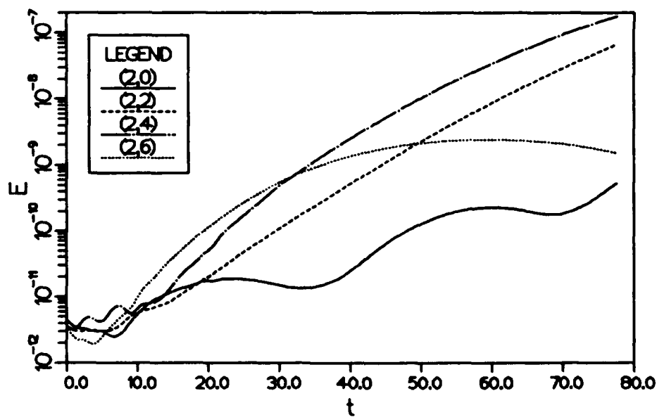
Figure 5.41 Growth in energy for selected modes from the simulation beginning with random numbers at M_1 = 1.05
