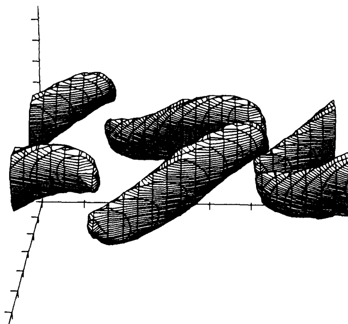
Figure 5.47 Surface of constant pressure, showing structure developed from a pair of equal and opposite oblique waves.
