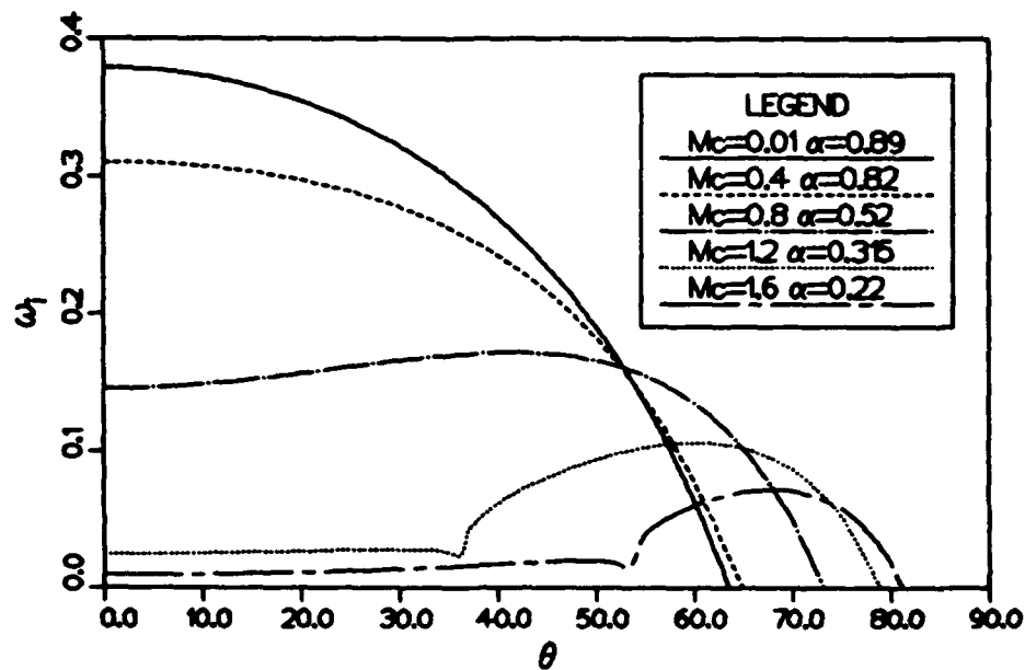
Figure 2.10 Variation of temporal amplification rate with angle of disturbance for the hyperbolic tangent velocity profile.
