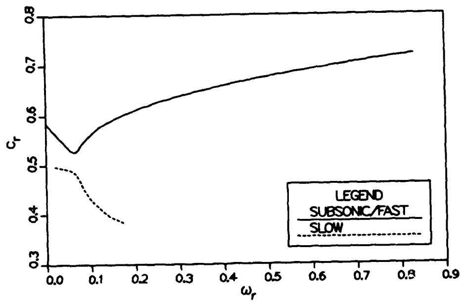
Figure 2.18 Phase speeds of supersonic modes against frequency.
