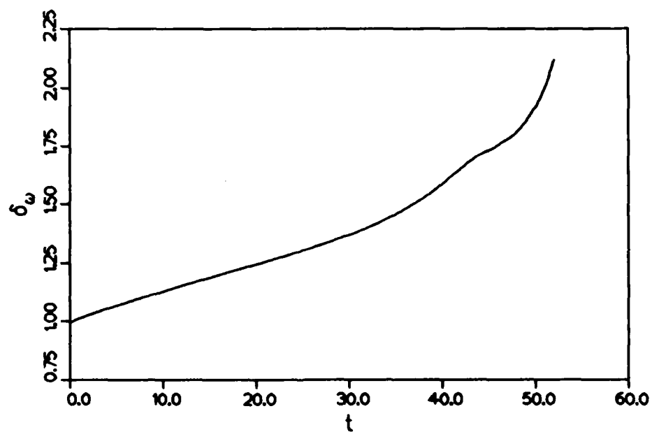
Figure 5.58 Growth in vorticity thickness for the simulation beginning with purely random initial conditions (a) regular vorticity thickness, (b) vorticity thickness based on mass-weighted velocity profile.
