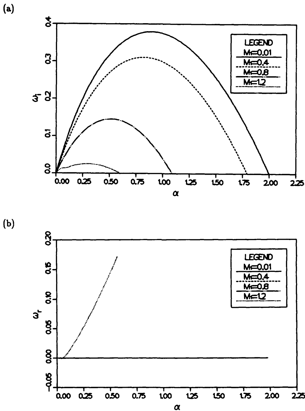
Figure 2.6 Effect of Mach number M_1 on the temporal eigenvalue (a) \omega_i , (b) \omega_r .
