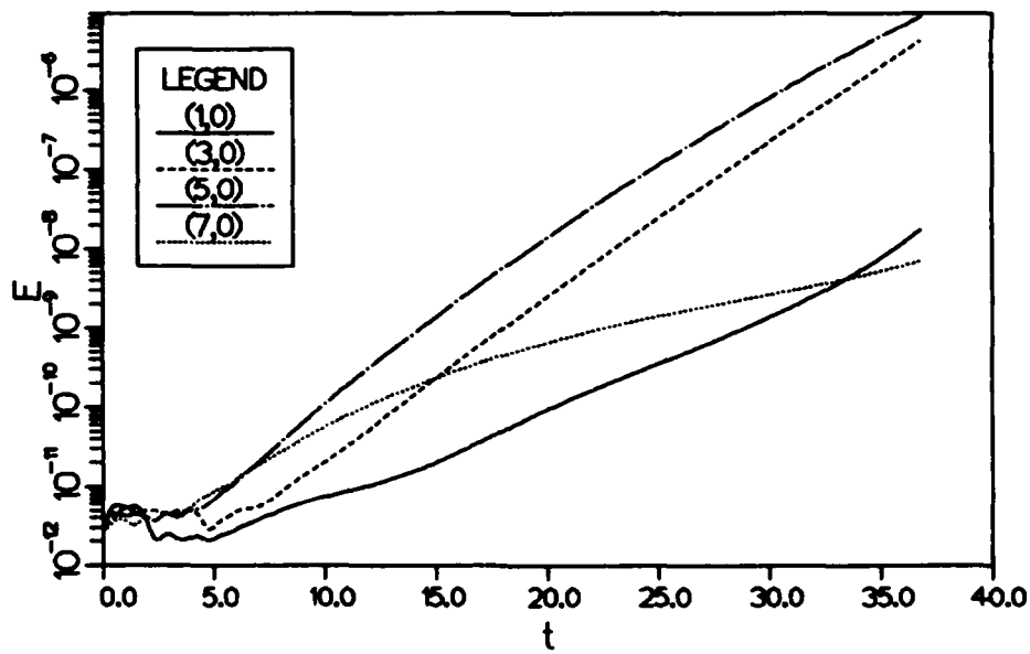
Figure 5.39 Growth in energy for selected modes from the simulation beginning with random numbers at M_1 = 0.4
