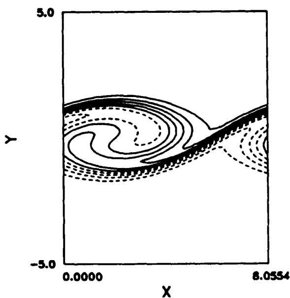
Figure 4.3 Developed structure at M_1 = 0.4 , Re = 100 (a) mixture fraction (b) vorticity.
