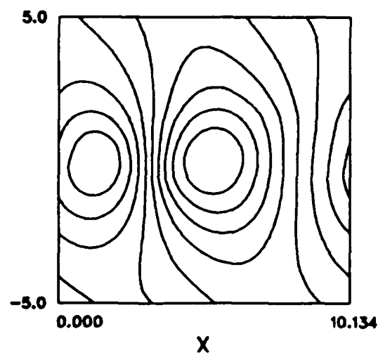
Figure 4.38 Convection of structure at T_2 = 5 shown by pressure contours (a) t = 0.0 , (b) t = 26.4 .
