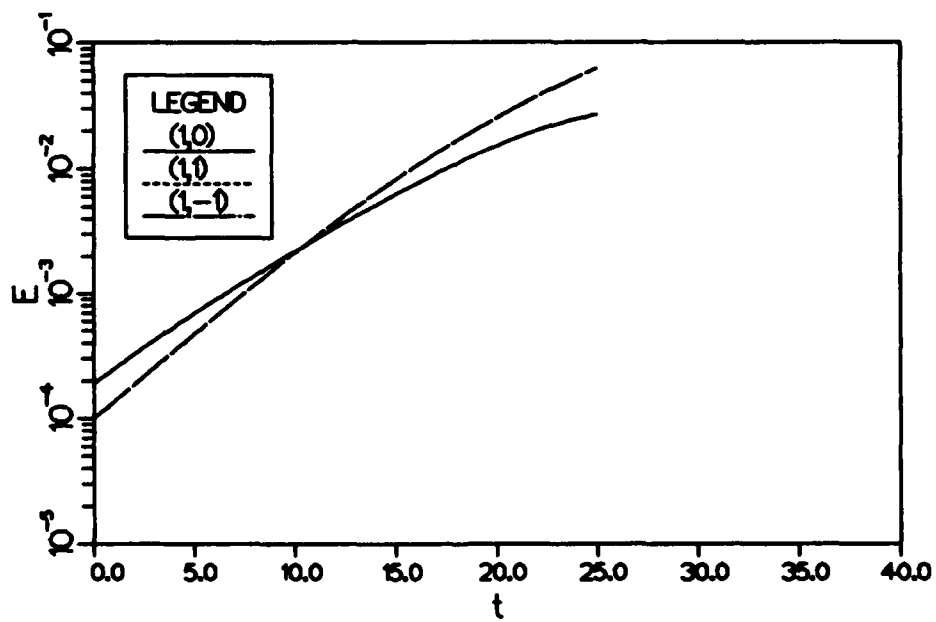
Figure 5.36 Growth in energy for the bulging instability mode at M_1 = 0.8 .
