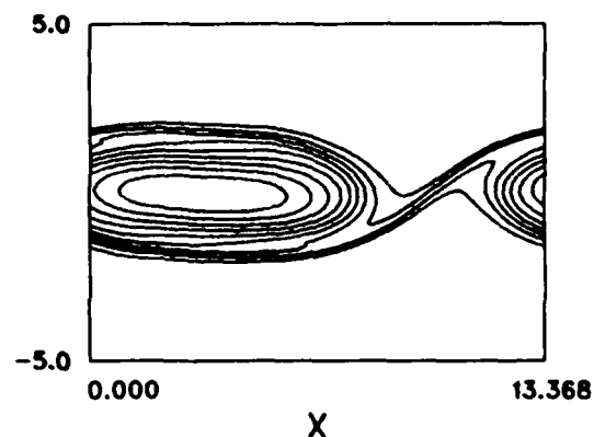
Figure 4.13 Developed structure at M_1 = 0.8 (a) mixture fraction, (b) pressure, (c) \omega_z , (d) \omega_z/\rho .
