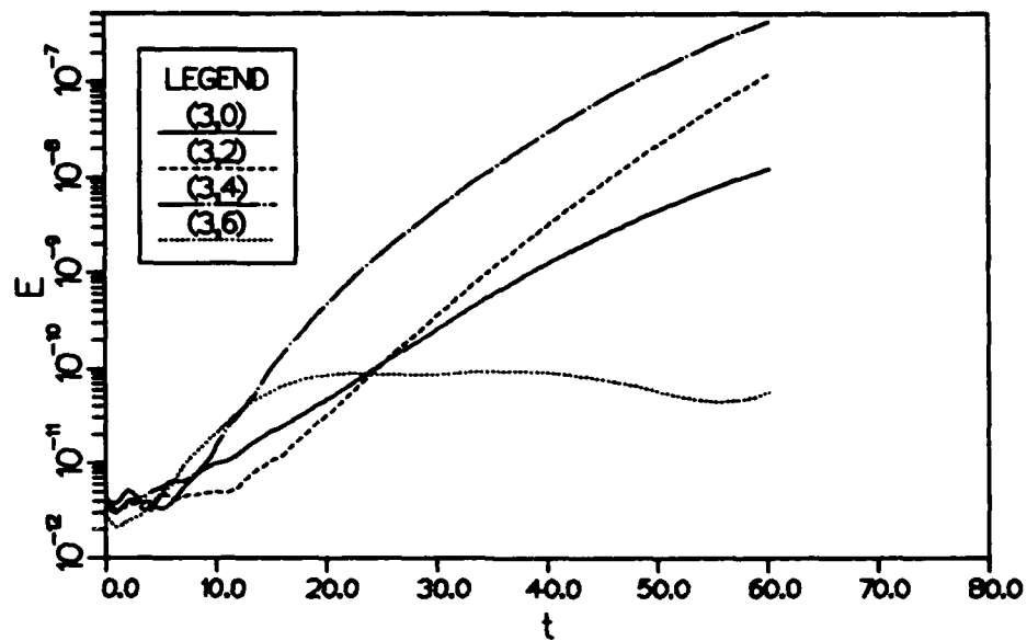
Figure 5.40 Growth in energy for selected modes from the simulation beginning with random numbers at M_1 = 0.8
