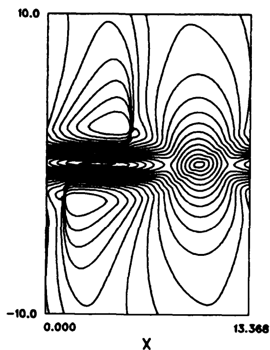
Figure 4.39 Embedded shock waves (a) pressure contours, (b) Mach contours M = \sqrt{u^2 + v^2}/c .
