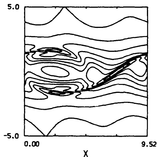
Figure 4.29 Plot of strain rate and mixture fraction at M_1 = 0.6 , t = 18.2 (a) mixture fraction, (b) strain rate S .
