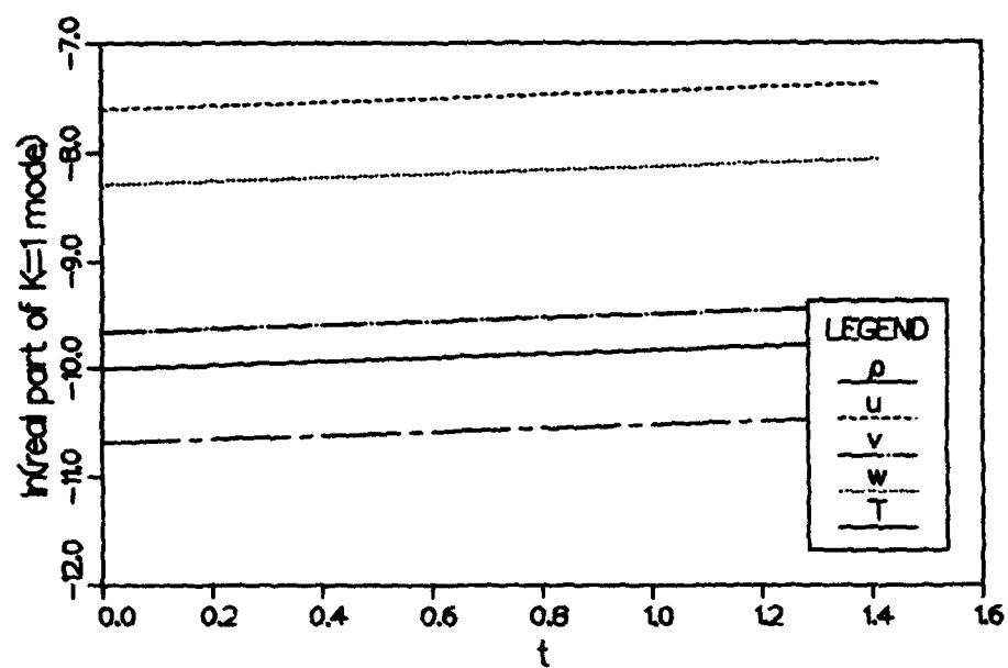
Figure 3.2 Check on linear growth rates for the inviscid eigenfunctions in the three-dimensional code.
