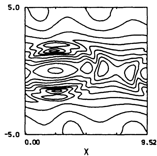
Figure 4.30 Plot of strain rate and mixture fraction at M_1 = 0.6 , t = 24.0 (a) mixture fraction, (b) strain rate S .
