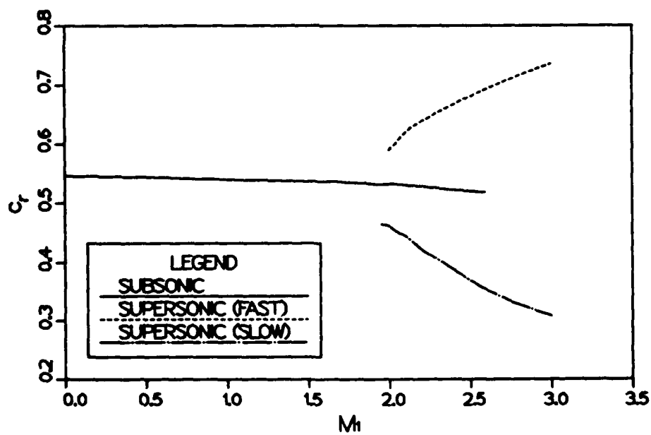
Figure 2.16 Phase speeds of subsonic and supersonic modes.
