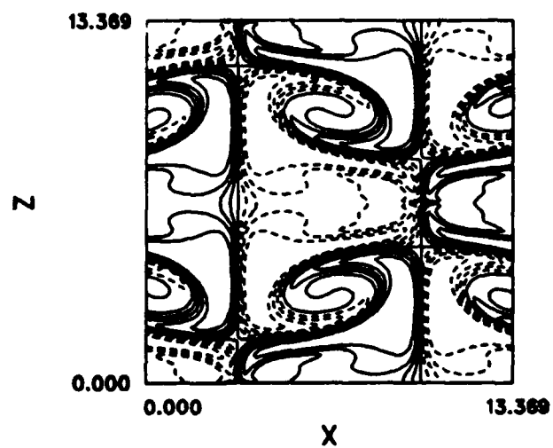
Figure 5.49 Mixture fraction cut through the x - z plane at y = 0 .
