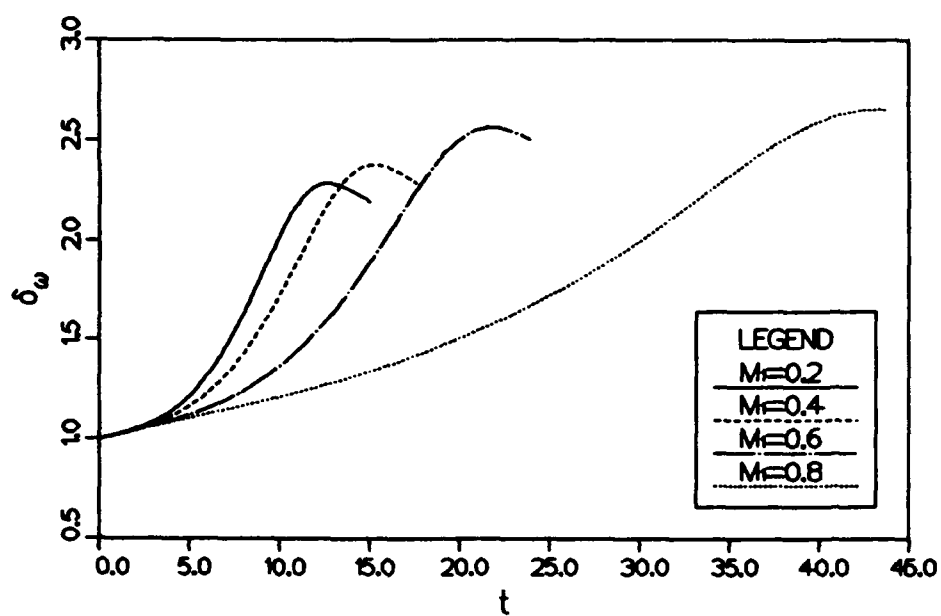
Figure 4.5 Effect of Mach number M_1 on the growth of the fundamental, most amplified disturbance.
