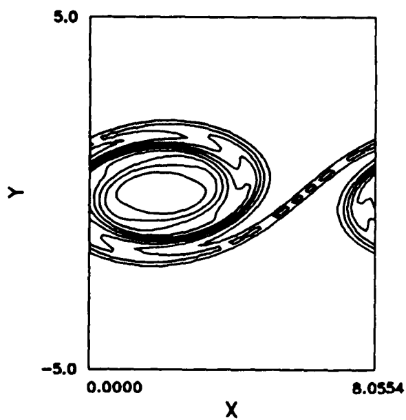
Figure 4.11 Developed structure at M_1 = 0.4 (a) mixture fraction, (b) pressure, (c) \omega_z , (d) \omega_z/\rho .
