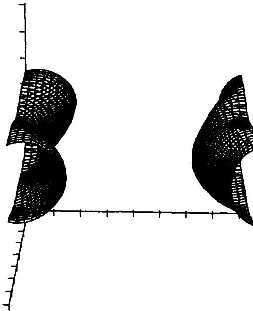
Figure 5.9 Surface of constant pressure showing the rotational region in the structure developing from the translative instability at M_1 = 0.4 .
