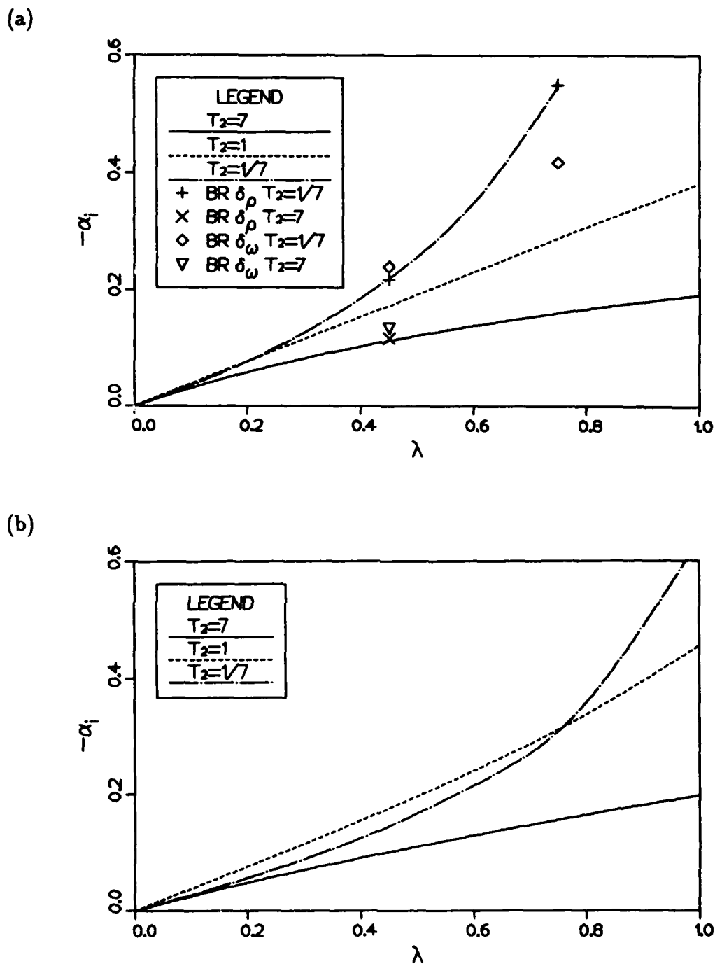
Figure 2.3 Spatial amplification rate plotted against \lambda = (U_1^* - U_2^*)/(U_1^* + U_2^*) , showing the combined effects of velocity and density ratio: (a) profiles from boundary-layer equations, (b) hyperbolic tangent.
