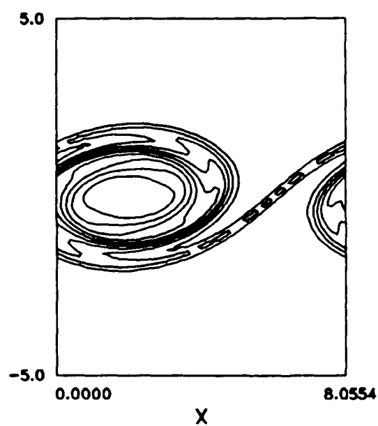
Figure 3.5 Developed structure for L_y = 10 (a) mixture fraction (b) vorticity.
