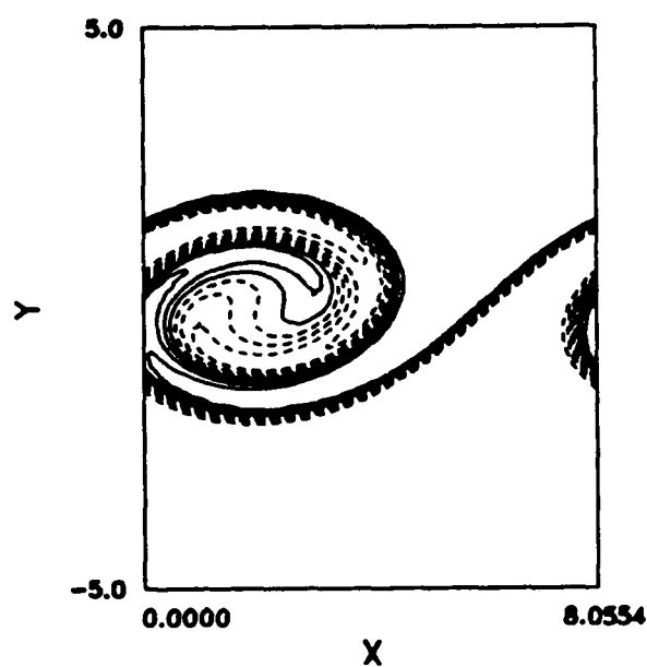
Figure 4.4 Developed structure at M_1 = 0.4 , Re = 800 (a) mixture fraction (b) vorticity.
