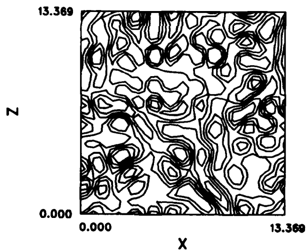
Figure 5.53 Simulation with random initial conditions at time t = 0 (a) carpet plot of mode energies, (b) pressure cut at y = 0 .
