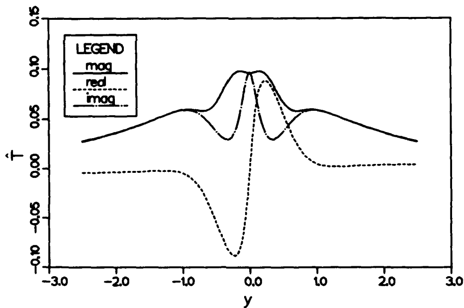
Figure 2.21 Eigenfunctions from temporal stability analysis at M_1 = 0.6 (a) \hat{u} , (b) \hat{v} , (c) \hat{\rho} , (d) \hat{T} .
