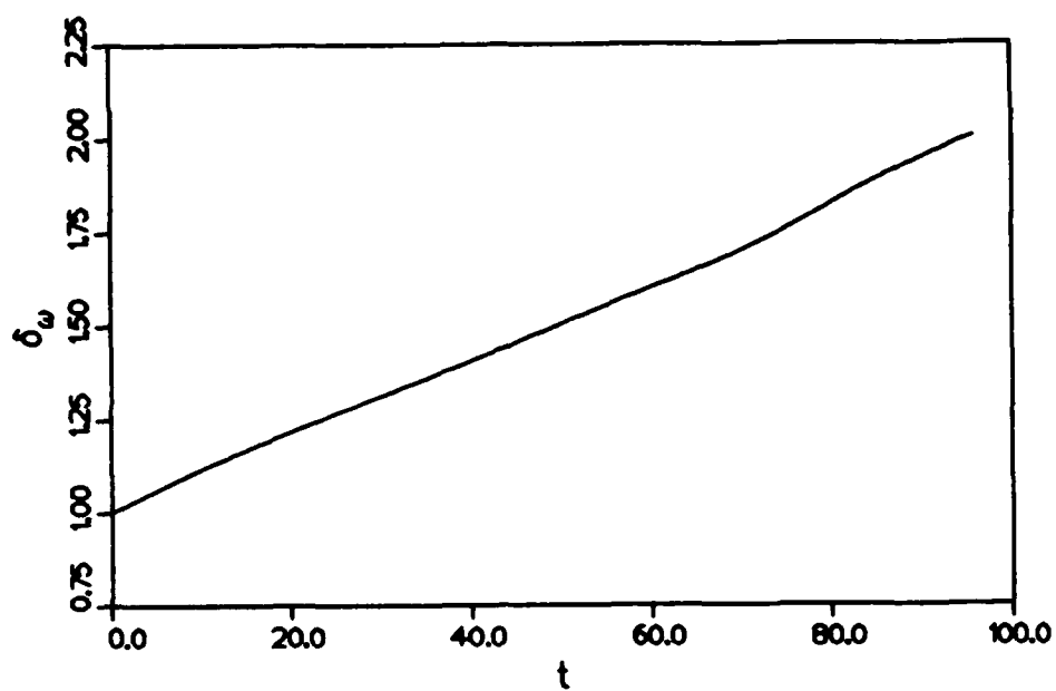
Figure 4.41 Growth of vorticity thickness for supersonic instability mode.
