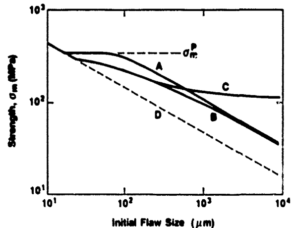
Figure 7 Predicted strength plotted against initial flaw size ( c_0 for microcracks, h_0 for pores) for alumina material in Fig. 2: A, microcracks with full T -curve history, B, microcracks with T -curve influence only after extension from c_0 , C, pores with T -curve influence after extension from h_0 , D, microcracks with no influence of T -curve at any stage of growth. Note well-defined plateau level at \sigma_m^P is fully achieved only by flaw A
