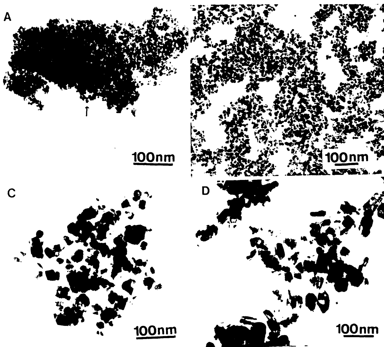
Fig. 3. Transmission electron micrographs of \text{ZrO}_2 powders by hydrothermal treatment: (A) Very poorly crystalline monoclinic and tetragonal \text{ZrO}_2 along with amorphous \text{ZrO}_2 (arrow) from \text{ZrO}_2 gel at 250^\circ\text{C}/4\text{MPa}/5 hrs. (B) Monoclinic \text{ZrO}_2 at 450^\circ\text{C}/100\text{MPa}/3 hrs. (C) Monoclinic and tetragonal \text{ZrO}_2 powder from \text{ZrO}_2 gel (slow hydrolysis in air) at 500^\circ\text{C}/100\text{MPa}/24 hrs. (D) Monoclinic \text{ZrO}_2 from \text{ZrO}_2 precipitate (in NaOH) at 500^\circ\text{C}/100\text{MPa}/24 hrs.
