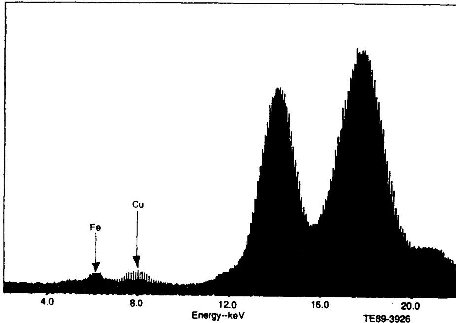
Figure 28. New oil and 50 ppm copper total spectra 8 gpm.
