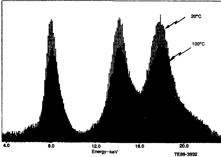
Figure 34. Copper foil total spectra for 100°C and 20°C.
