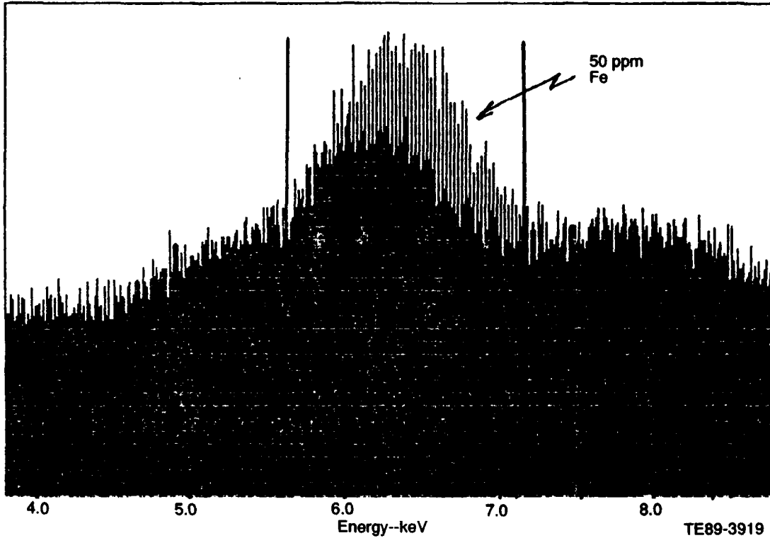
Figure 21. New oil and 50 ppm iron spectra - 8 gpm flow rate.
