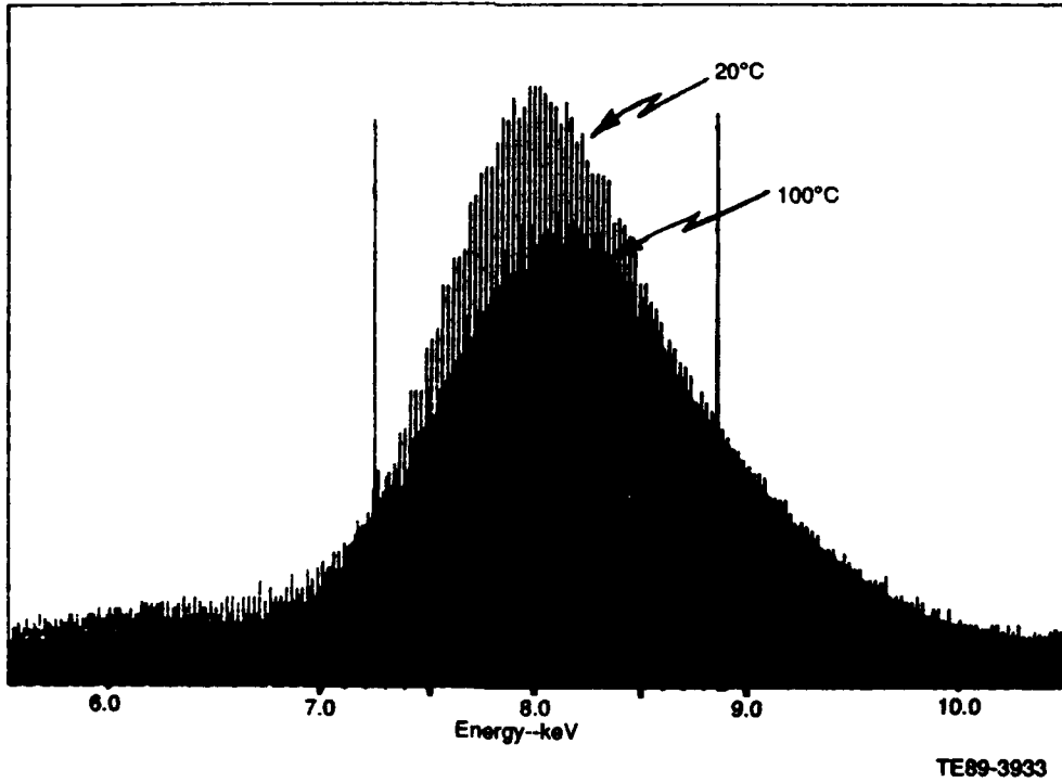
Figure 35. Copper foil spectra for 100°C and 20°C.
