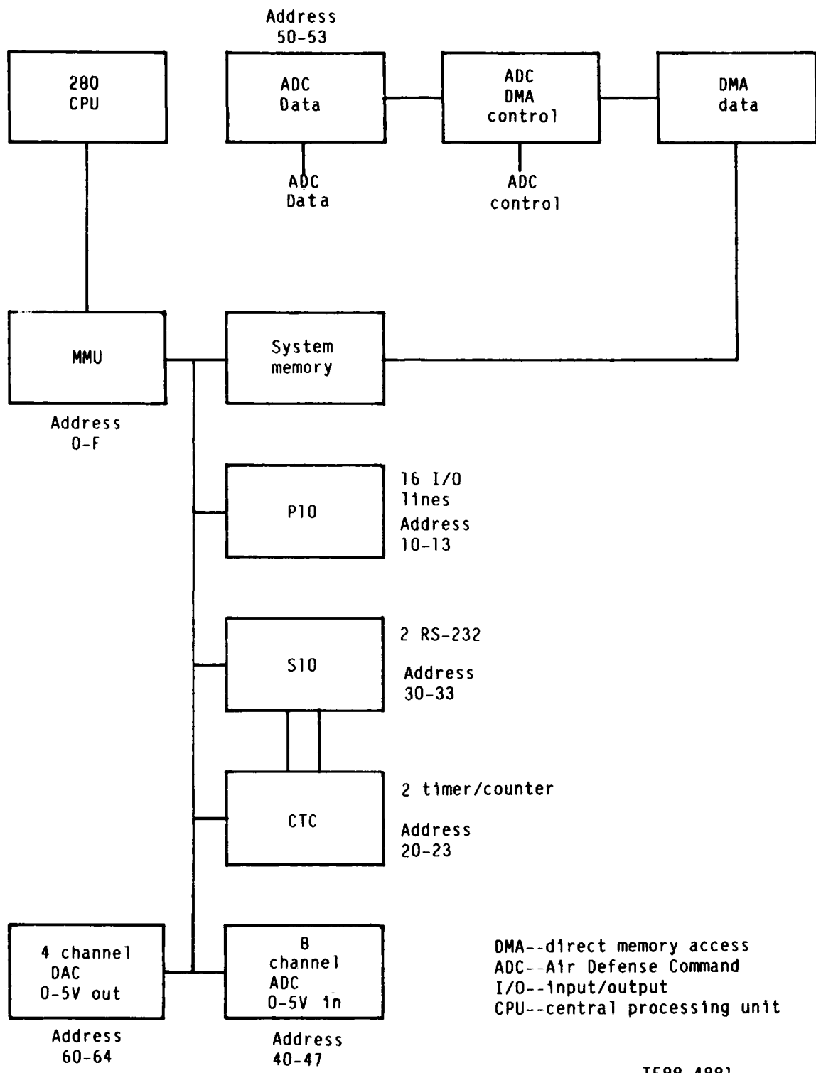
Figure 4. Data processing electronics block diagram.
