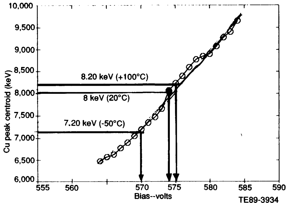
Figure 36. Copper peak centroid versus bias voltage.
