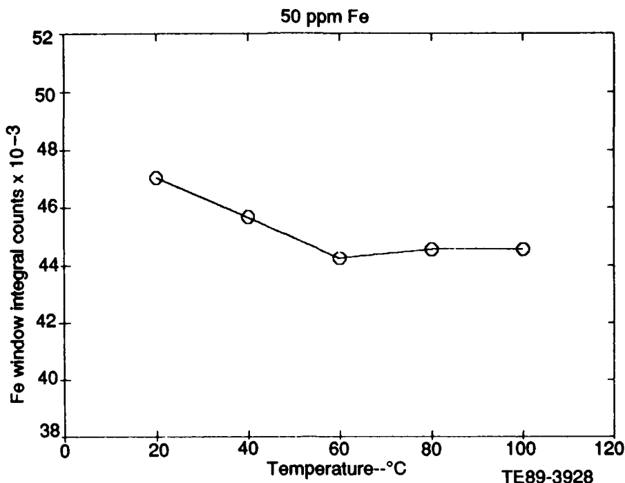
Figure 30. Iron counts versus oil temperature.
