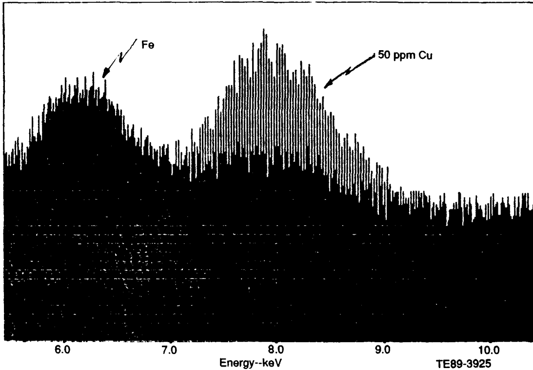
Figure 27. New oil and 50 ppm copper spectra - 8 gpm flow rate.
