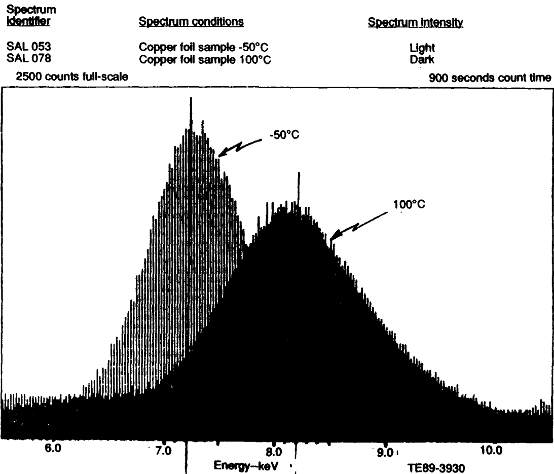
Figure 32. Copper foil spectra for 100^{\circ}\text{C} and -50^{\circ}\text{C} .
