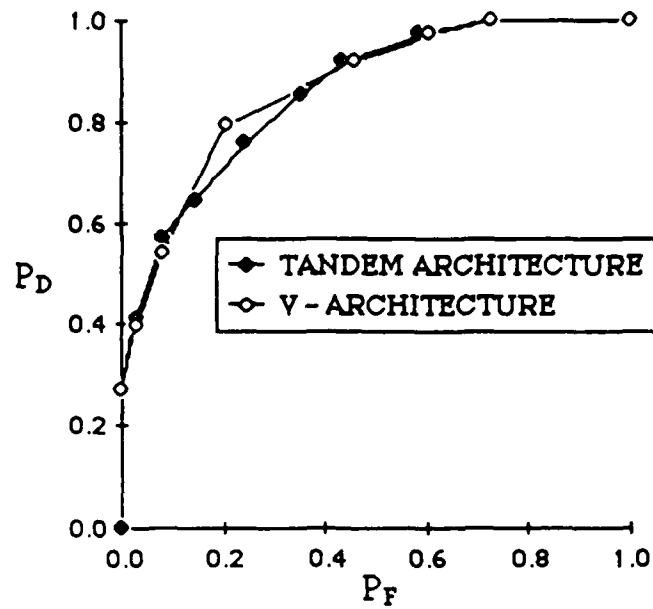
Figure 17(a). Team ROC Curves for DMs of Figure 16: No Dominant Architecture Exists
