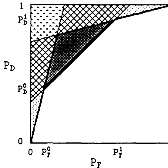
Figure C.2. The Six Cases for the Consulting DM
