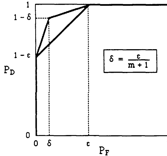
Figure 7. The DMs in Example 2
