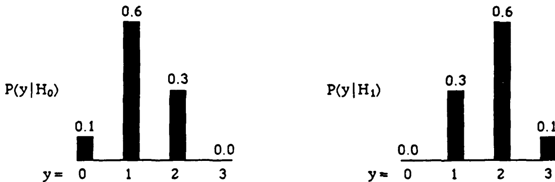
Figure 16. DM for which the Optimal Architecture Depends on \eta
