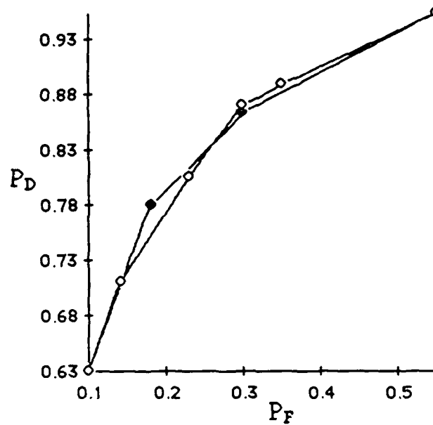
Figure 5(b). Close Up on Figure 5(a)
