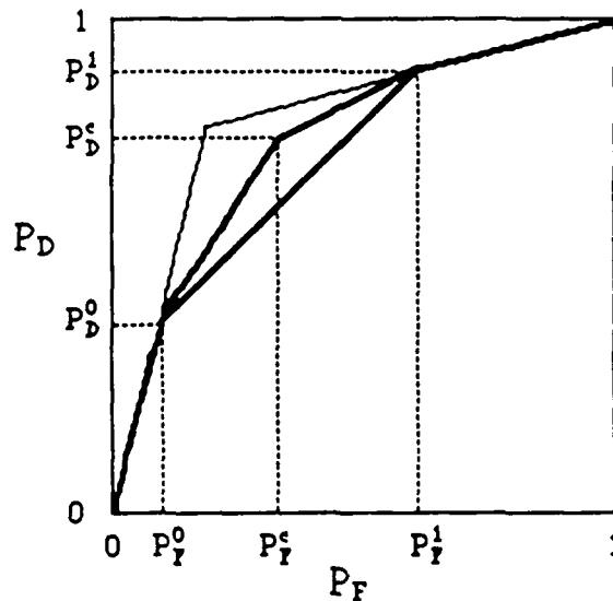
Figure C.3. The 'Restricted' DMs of the Analysis
