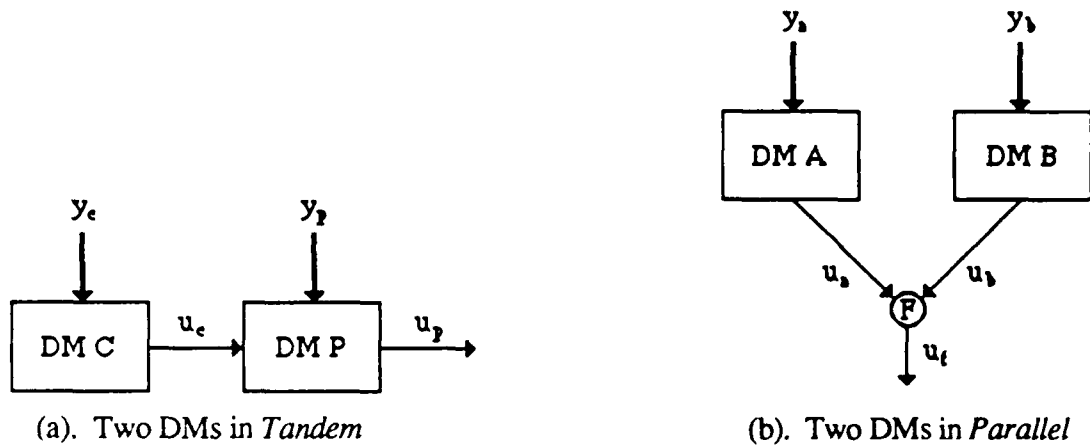
Figure 1. Architectures for Teams Consisting of Two DMs
