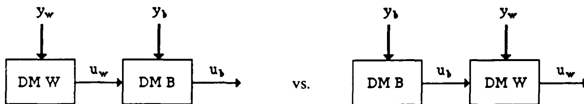
Figure 2. Different Configurations for the Two DM Tandem Team
