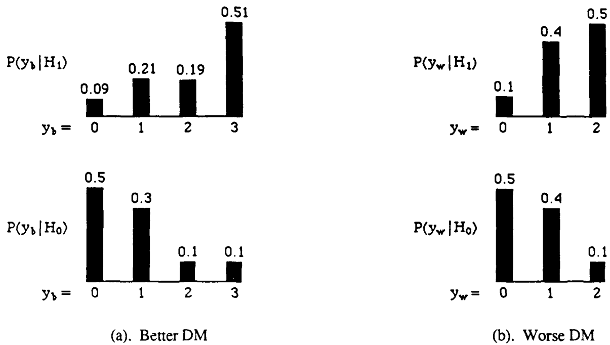
Figure 4. The Probability Distributions for the DMs of Figure 3
