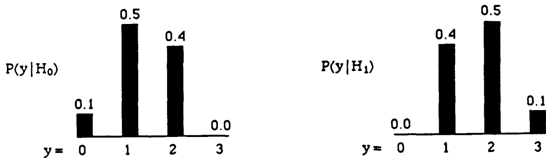
Figure 18. DM resulting in Dominant Tandem Architecture
