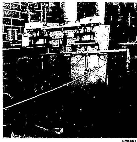
Figure 14. High Temperature Deflection Beam Test Fixture
