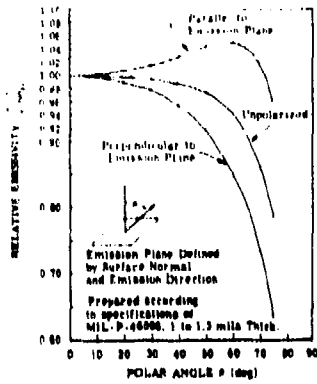
Polarized Emittance for O.D. Paint on Steel (9.96 \mu m)
