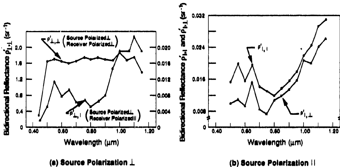
Figure 2-2. Spectral Bidirectional Reflectance for Green Paint (Sample No. 1027) for a Specular Geometry Where \theta_i = 55^\circ = \theta_r
