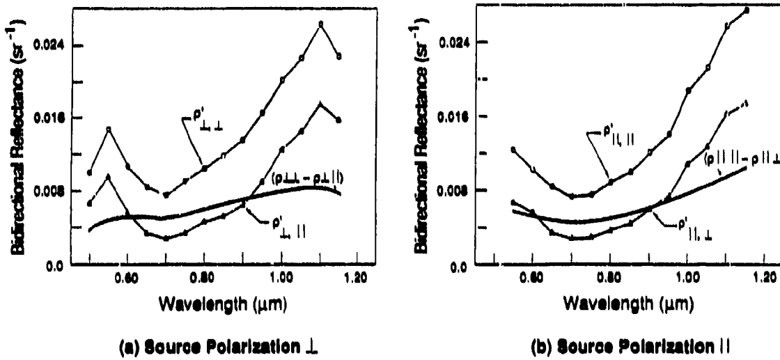
Figure 2-1. Spectral Bidirectional Reflectance for Green Paint for Normal Incidence and \theta_r = 50^\circ
