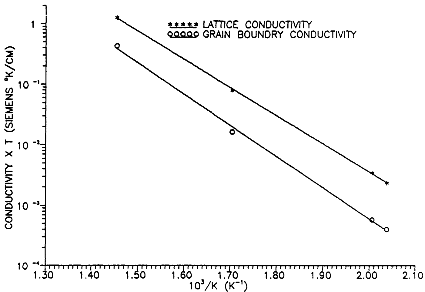
Figure 10. Conductivity \sigma T Vs. Temperature, PO_2 = 0.1 Oxide B1
