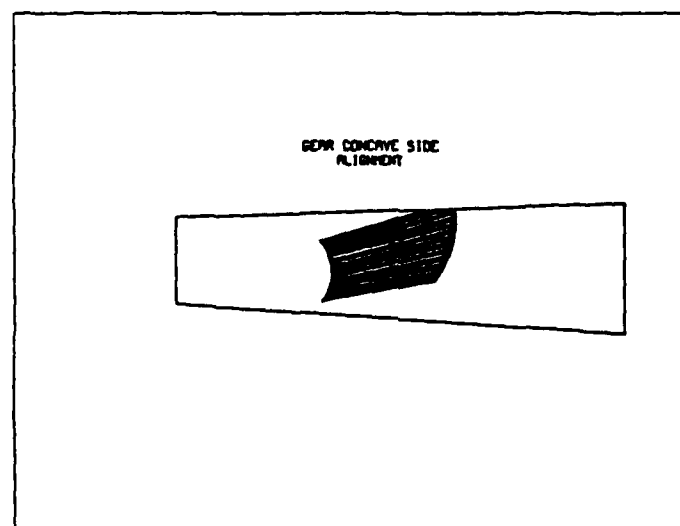
Figure 30: Straight-edged blade, gear concave side, alignment.
