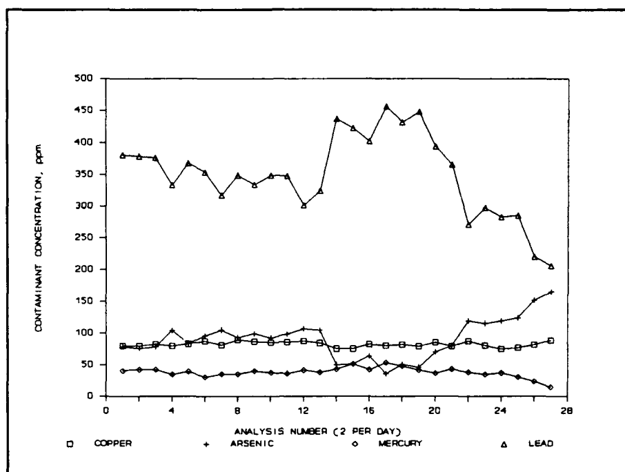
Figure 12. Field Analysis of Water Standard AM-14. CSI (Multivariate) Calibration.
