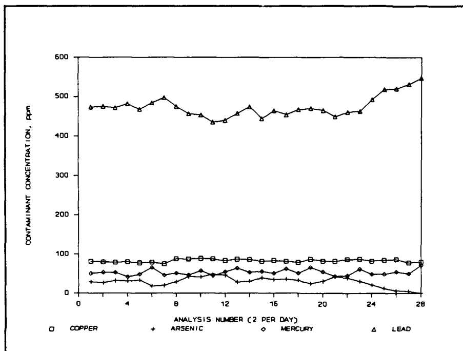
Figure 10. Laboratory Analysis of Water Standard AM-14. CSI (Multivariate) Calibration.
