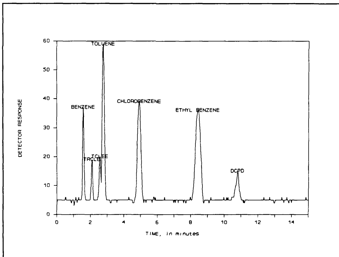
Figure 2. Detector Trace from Scentograph Portable GC. [TRCLE: trichloroethylene; TCLEE: tetrachloroethylene; DCPD: dicyclopentadiene.]
