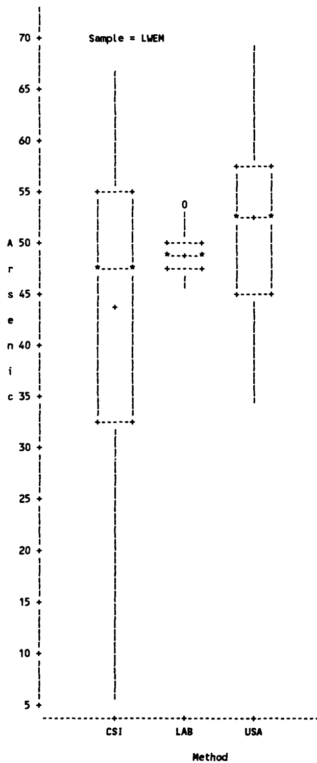
Fig. 1.3 Arsenic measurements ( \mu\text{g/mL} ) for Sample LWEM.
