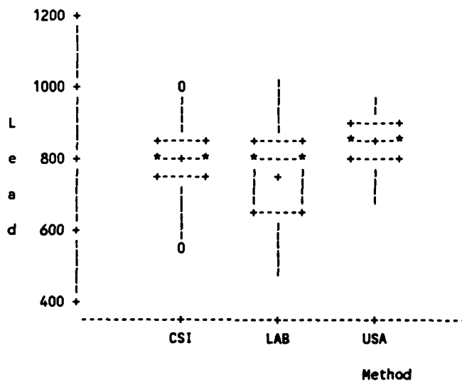
Fig. III.2 Lead measurements ( \mu\text{g/g} ) for Sample 2-8.
