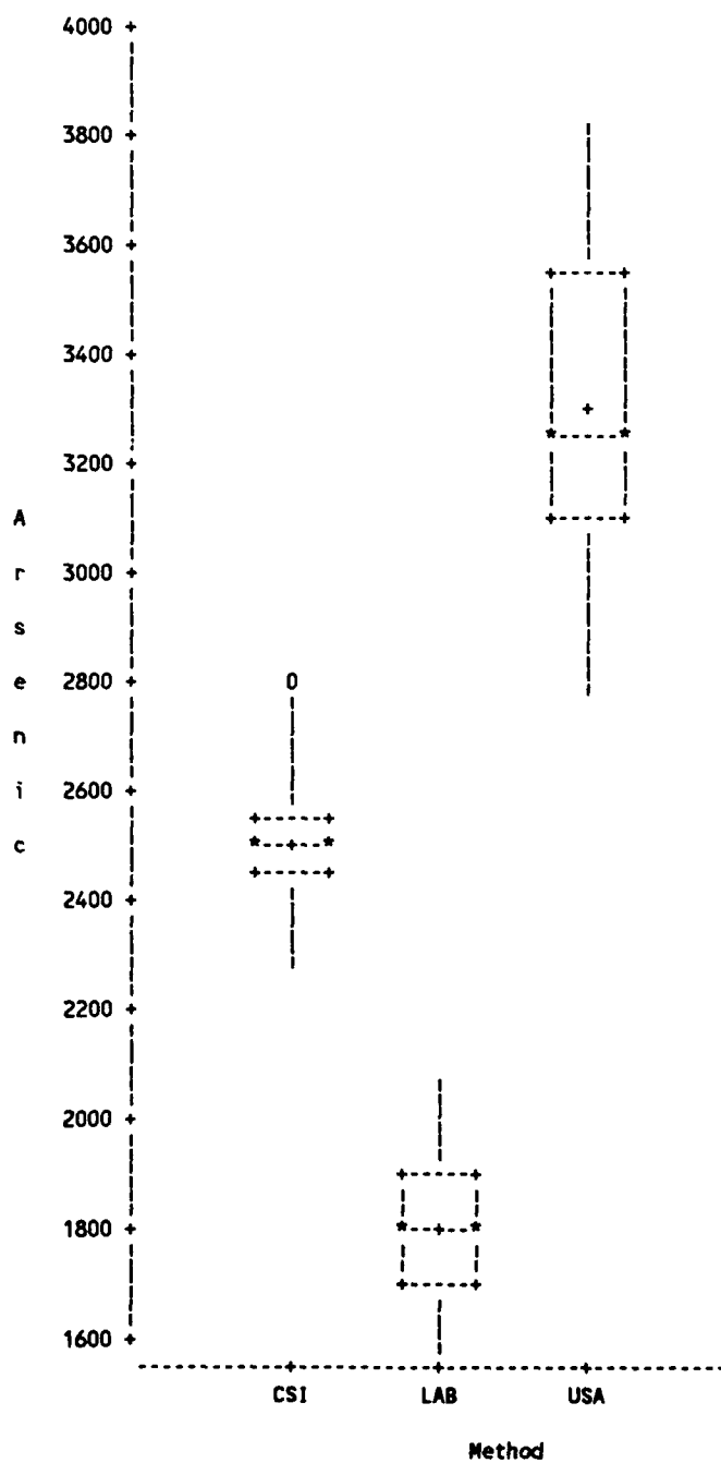
Fig. I.6 Arsenic measurements ( \mu\text{g/g} ) for Sample SILO.
