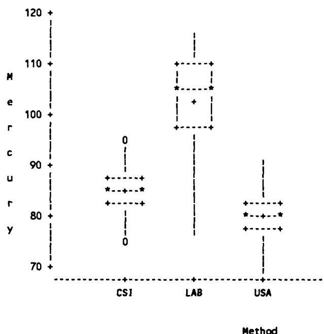
Fig. IV.1. Mercury measurements (µg/mL) for sample LWEM.
