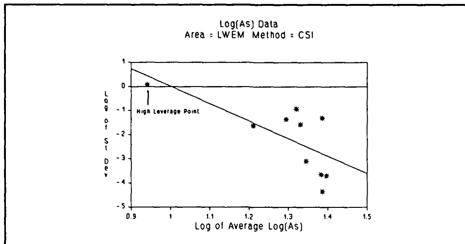
Fig. I.1 Equality of variance test for Sample LWEM and Method=CSI.
