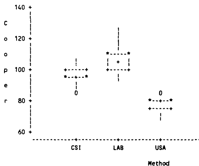
Fig. II.1 Copper measurements ( \mu\text{g/mL} ) for Sample LWEM.
