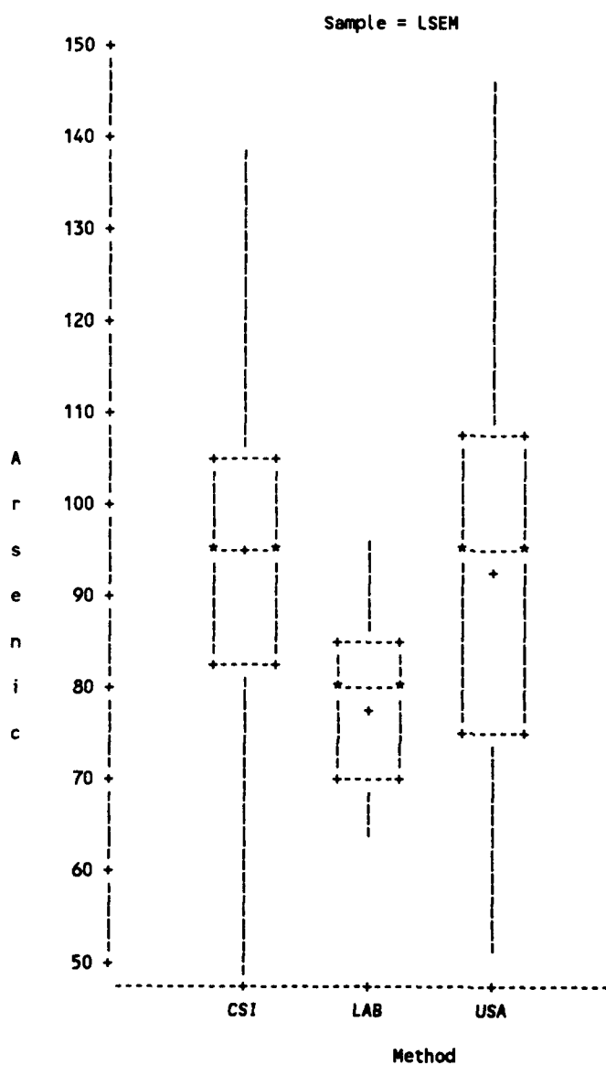
Fig. 1.5 Arsenic measurements ( \mu\text{g/g} ) for Sample LSEM.
