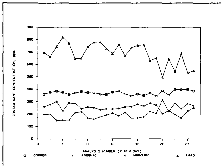
Figure 13. Field Analysis of Soil Standard SM-16. CSI (Multivariate) Calibration.
