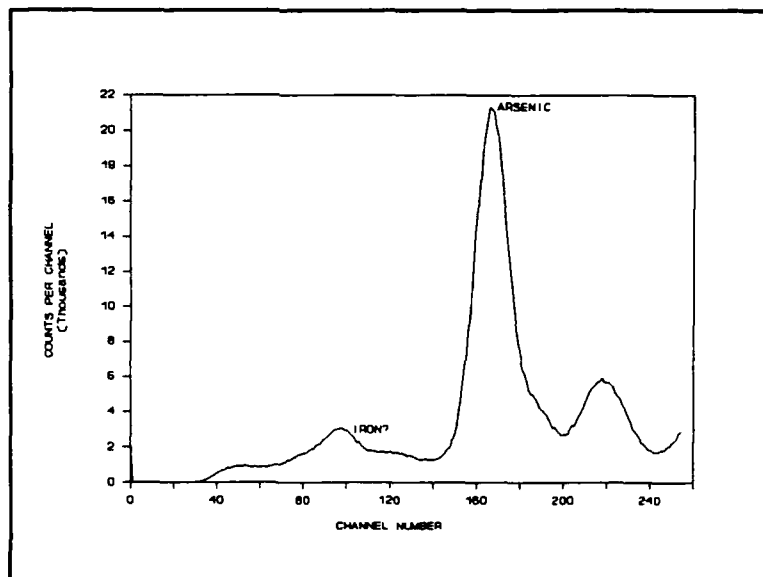
Figure 14. XRF Spectrum of Undiluted Water Sample Acquired from Sump Pit in Building 1703.
