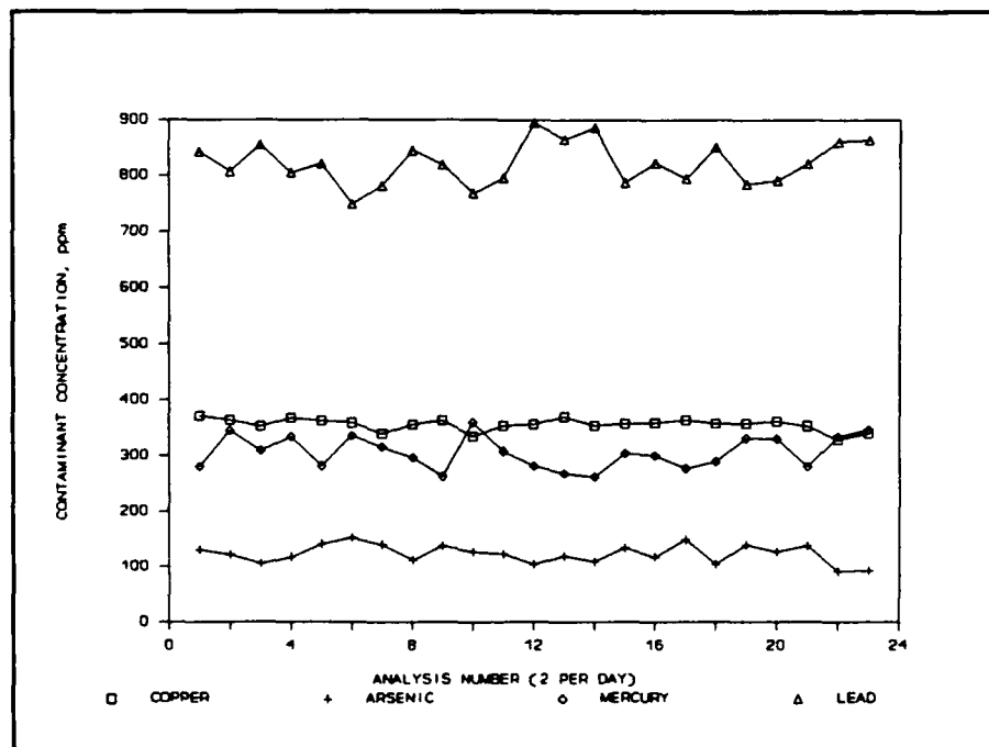
Figure 11. Laboratory Analysis of Soil Standard SM-16. CSI (Multivariate) Calibration.
