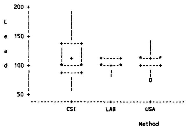
Fig. III.1 Lead measurements ( \mu\text{g/mL} ) for Sample LWEM.
