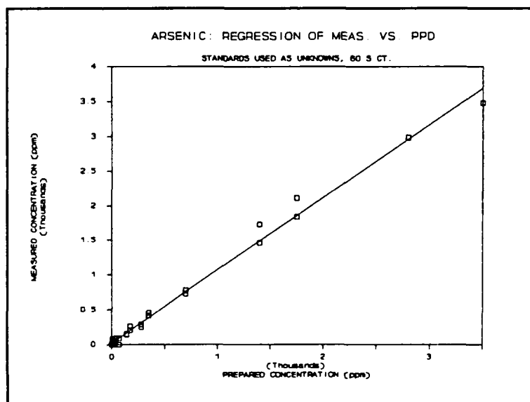
Figure 4. Comparison of Observed vs Spiked Concentrations for Arsenic in RMA Soil in the Presence of Copper, Lead, and Mercury.
