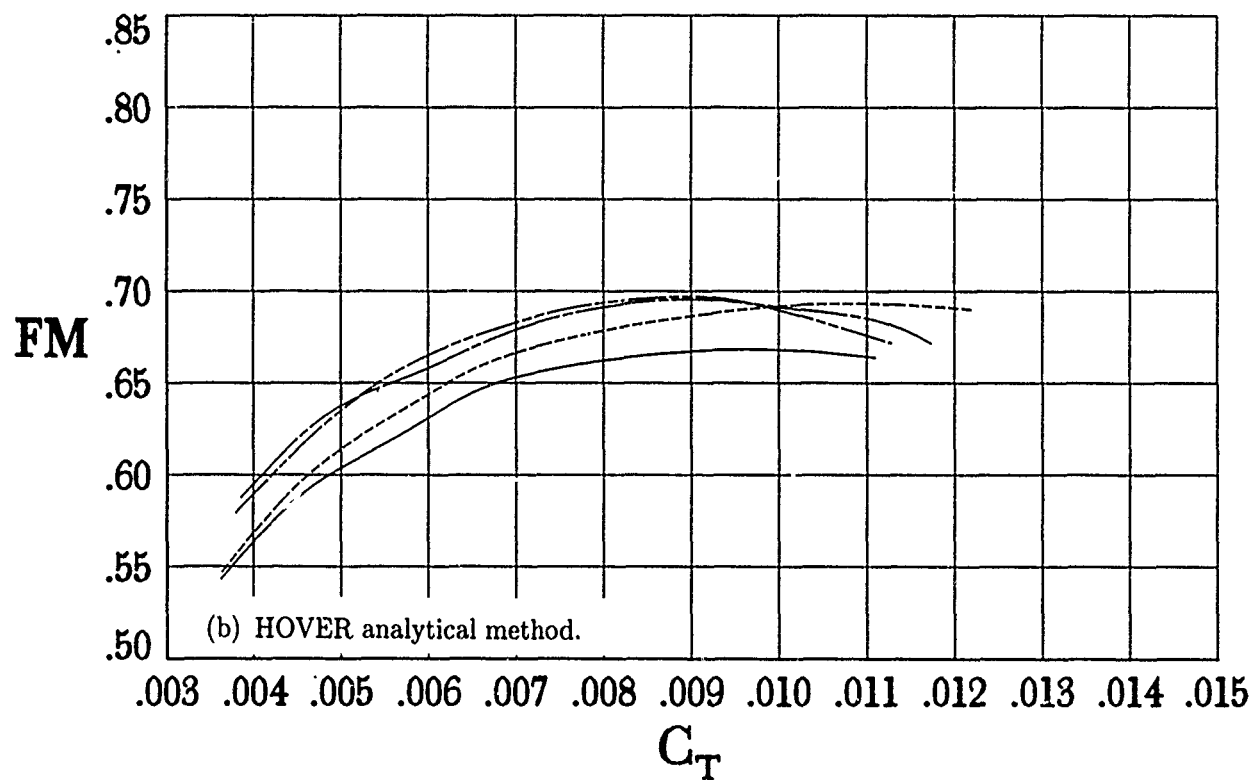
Figure 6. Comparison of trends predicted by analyses.
