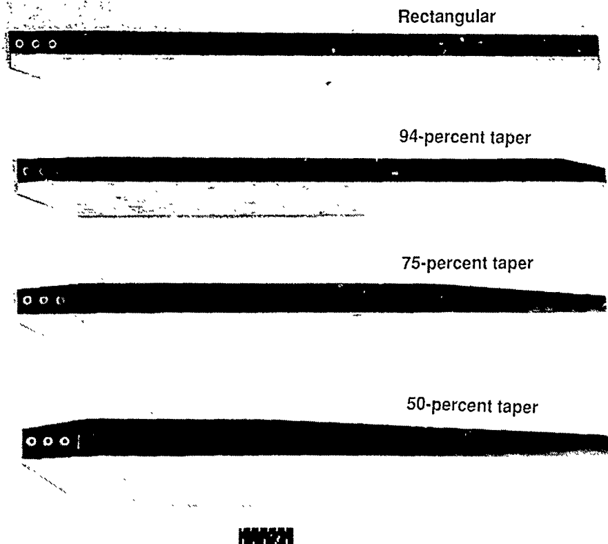
(a) Photograph of four blade planforms.
