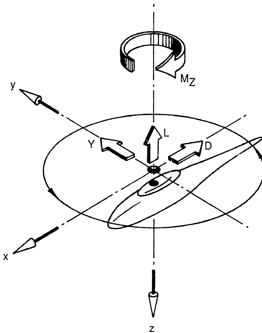
Figure 1. Axis system used for presentation of data. Arrows denote positive directions of forces, moments, and axes.
