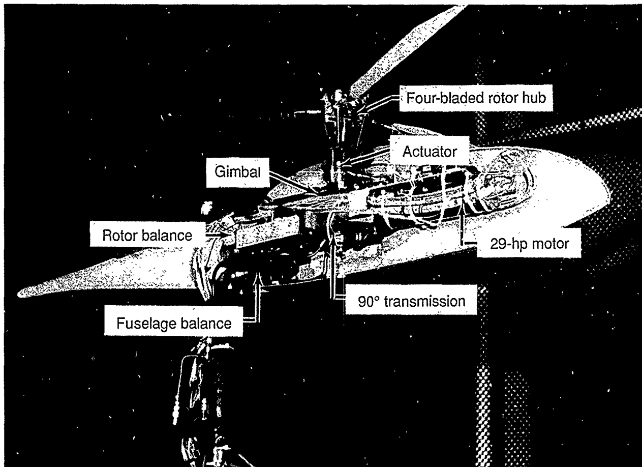
(b) Cutaway view of 2MRTS.
