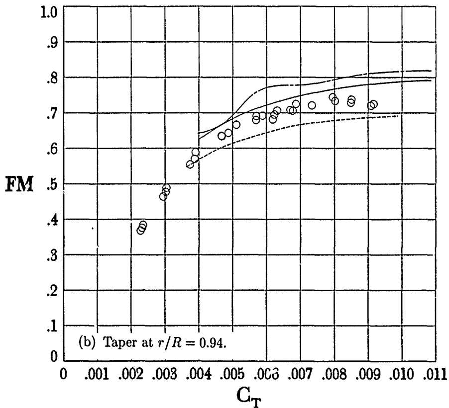
Figure 7. Comparison of prediction methods with experimental data.
