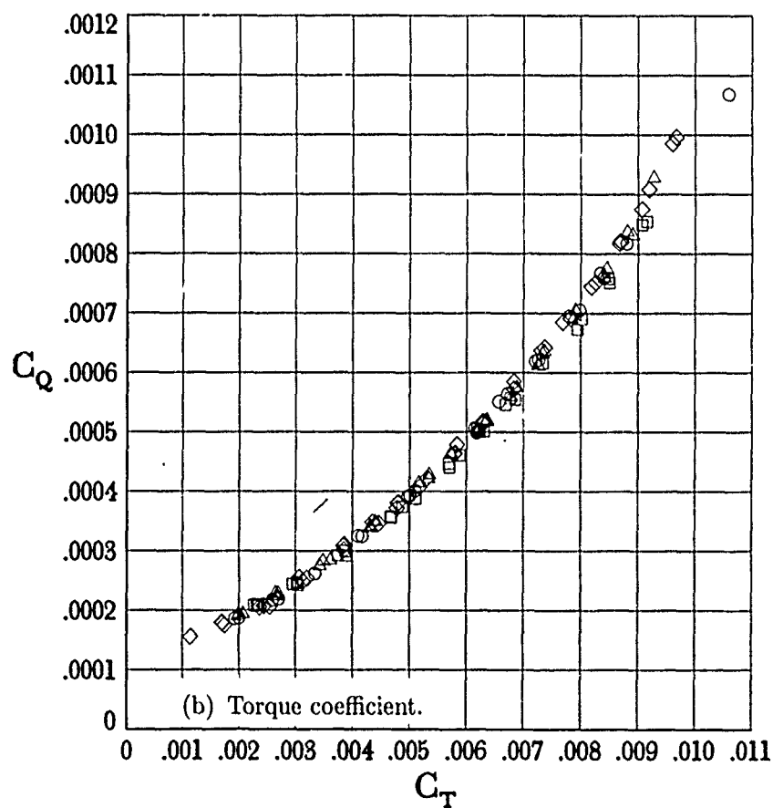
Figure 4. Comparison of basic aerodynamic characteristics of rotors.
