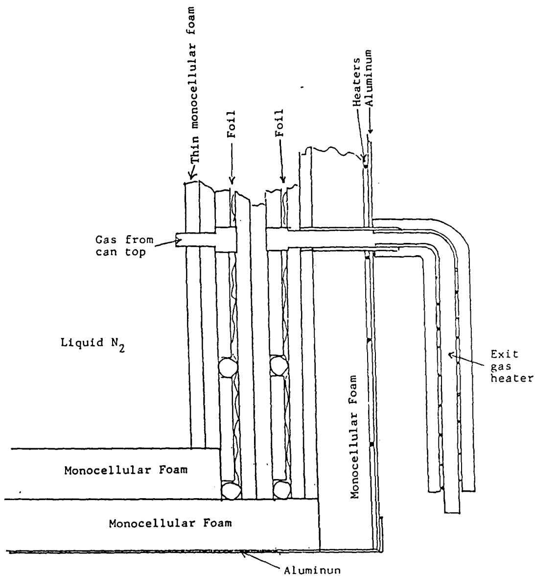
Fig. 2 Detail of Two-pass heat exchanger system
