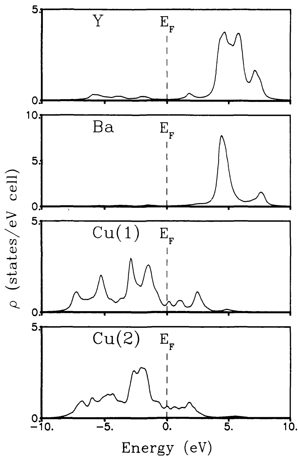
Fig. 4.5. Local densities of states for the metal atoms in \text{YBa}_2\text{Cu}_3\text{O}_7 .
