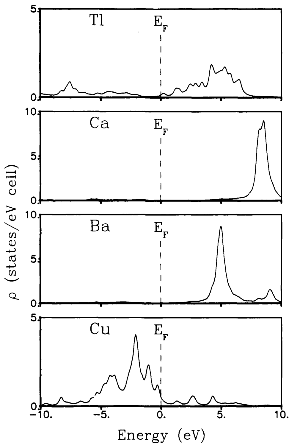
Fig. 4.17. Local densities of states for the metal atoms in \text{Tl}_2\text{CaBa}_2\text{Cu}_2\text{O}_8 .
