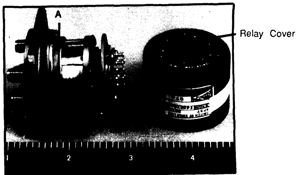
Figure 3.3-8 Military grade multi-pole RF relay
