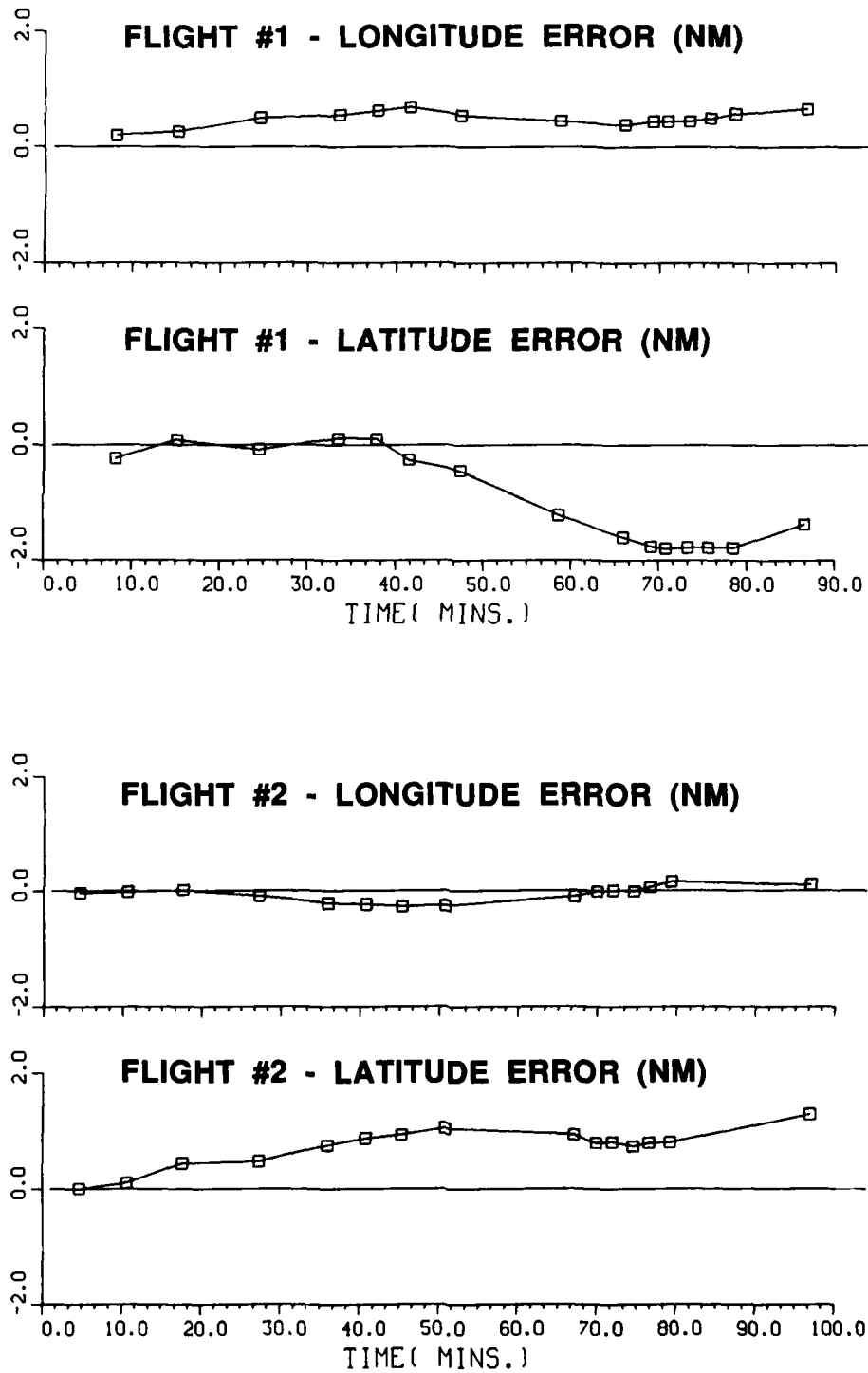
FIG. 4: IRS POSITION ERRORS
