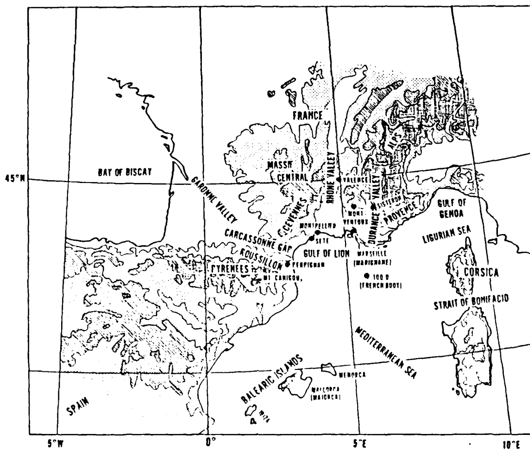
Figure 10. Locator map for the mistral (Brody and Nestor 1980)
