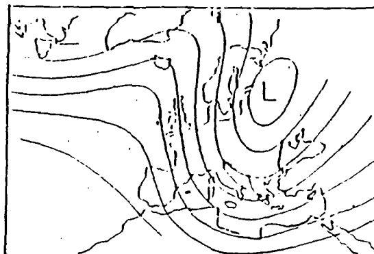
Figure 11-a. Upper-level flow pattern showing the British Air Ministry Type A.
