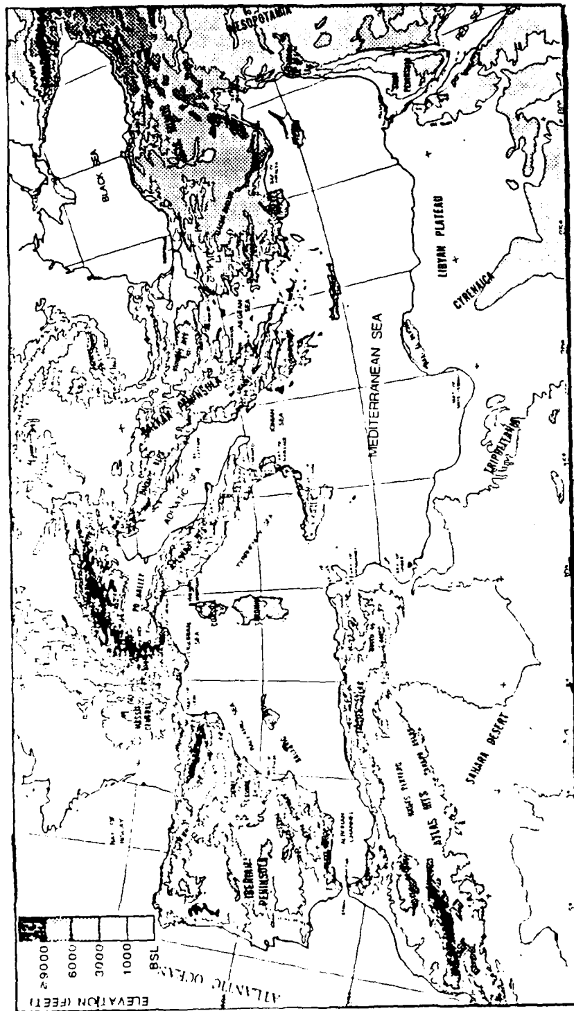
Figure 4. Map showing the topography of the Mediterranean area. (Reiter 1975)
