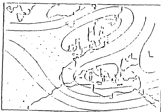
Figure 11-b. Upper-level flow pattern showing the British Air Ministry Type B.
