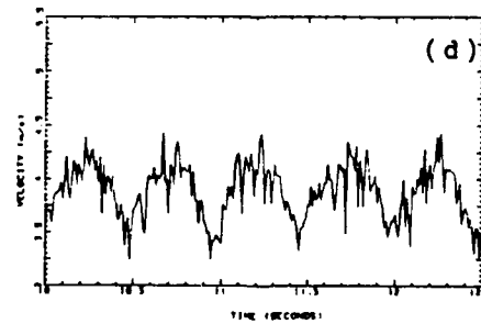
Figure 55. Instantaneous Velocity Traces (a) Re=3537 Str=0.0190 (b) Re=3453 Str=0.0195 (c) Re=3284 Str=0.0205 (d) Re=3158 Str=0.0213
