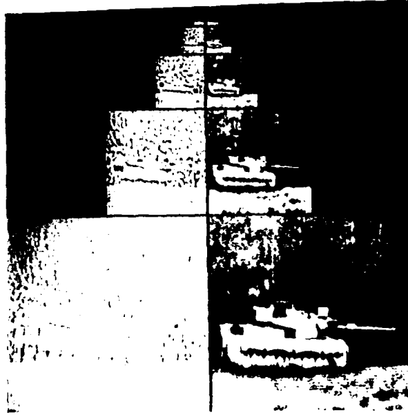
Fig. 11 The composite Gaussian ratio pyramid (left column) and the reconstructed composite Gaussian ratio pyramid (right column) of the CCD and FLIR images from Fig. 9a and b.
