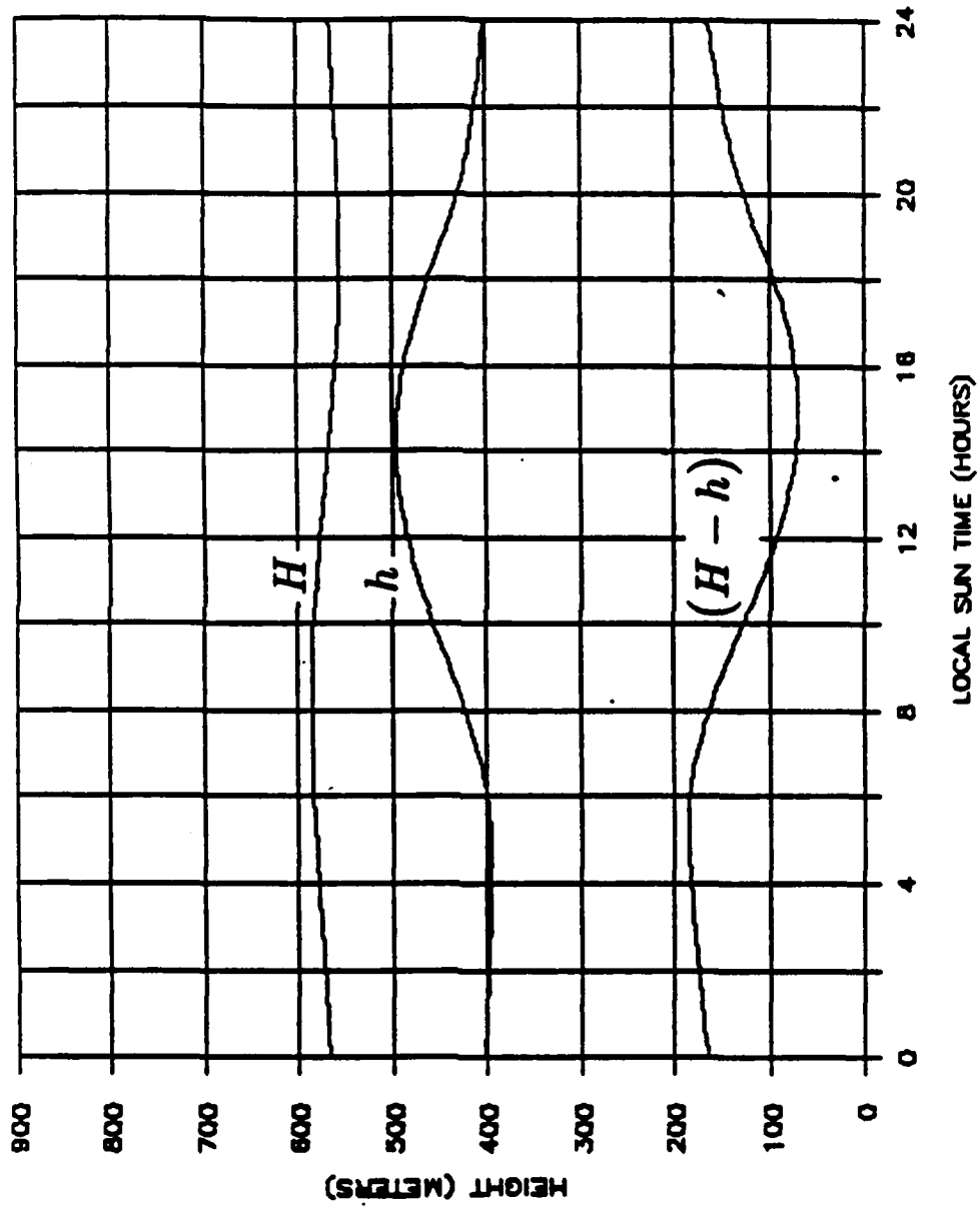
Figure 4.14: Cloud top, base and thickness curves as a function of time for the thin cloud case.
