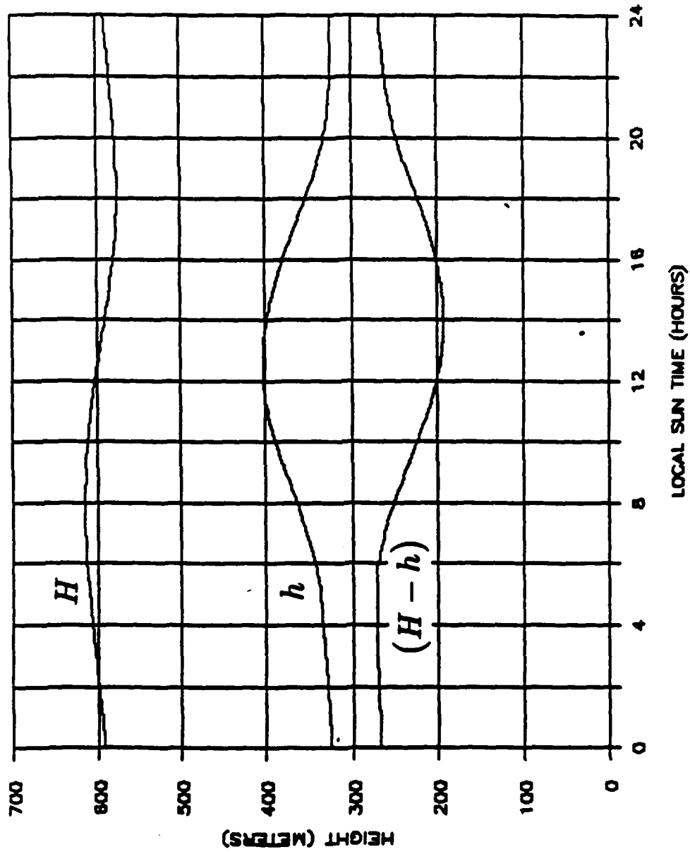
Figure 4.13: Cloud top, base and thickness curves as a function of time with an increased \mu' of 0.8.
