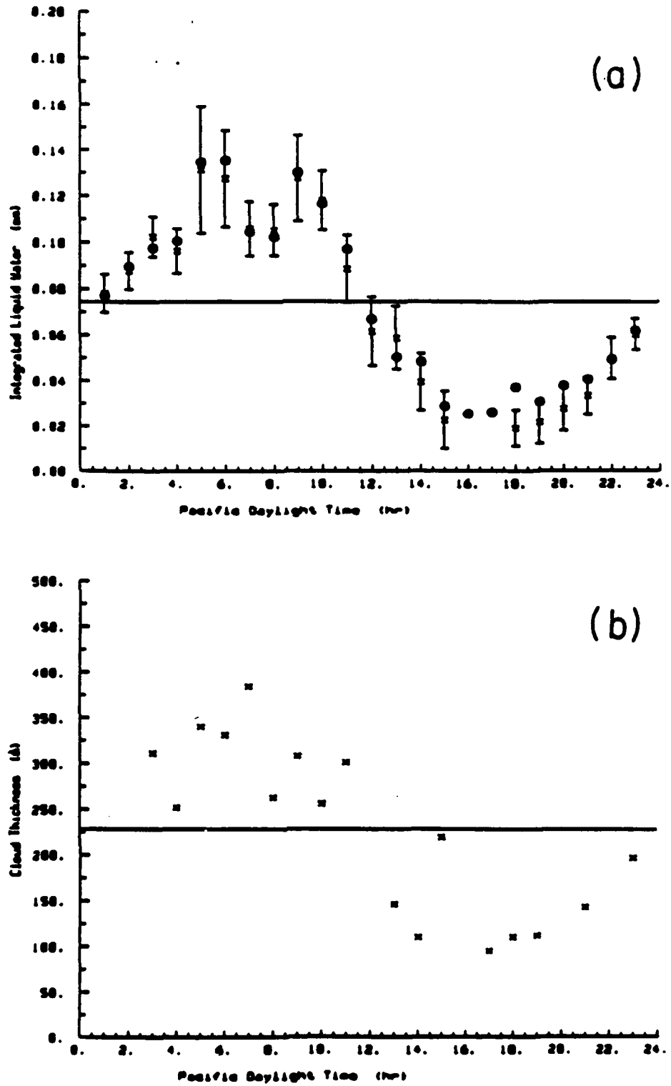
Figure 4.12: Observational values of (a) column liquid water as determined by the NOAA/WPL radiometer and (b) cloud thickness as determined by ceilometer and radiosonde data as a function of time (PST). From Davies and Blaskovic (1988).
